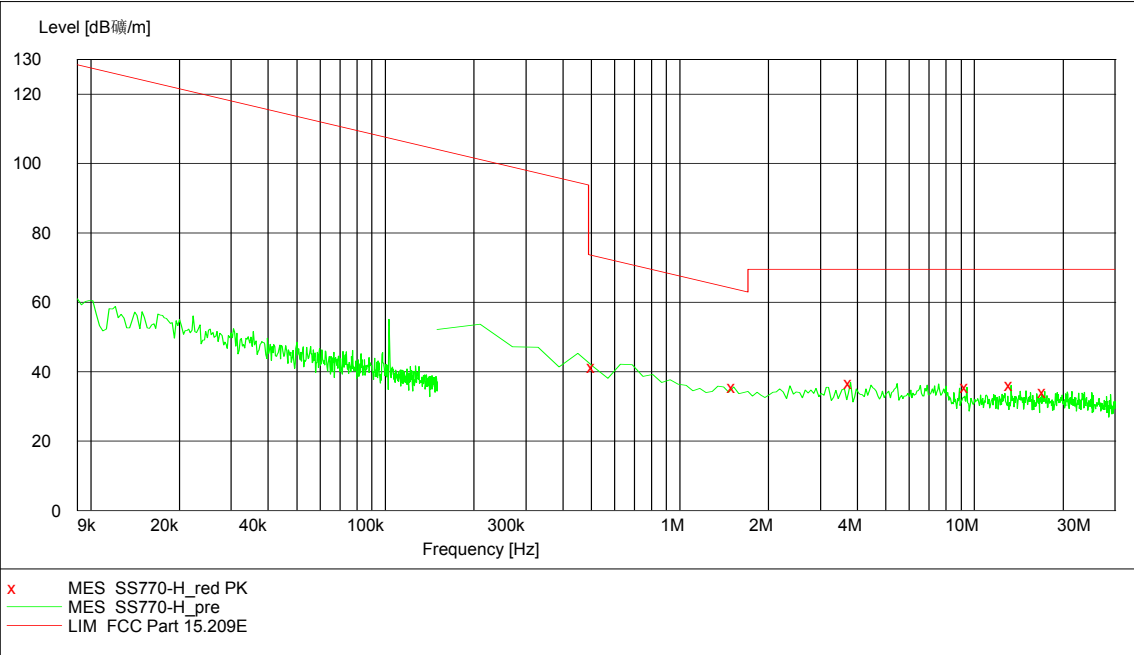
Radiated Emission Plot between 9 kHz ~ 30MHz (Vertical)
