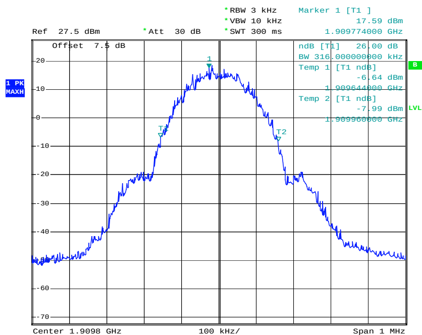
26dB Bandwidth Plot on Channel 810
