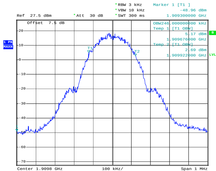
99% Occupied Bandwidth Plot on Channel 810
