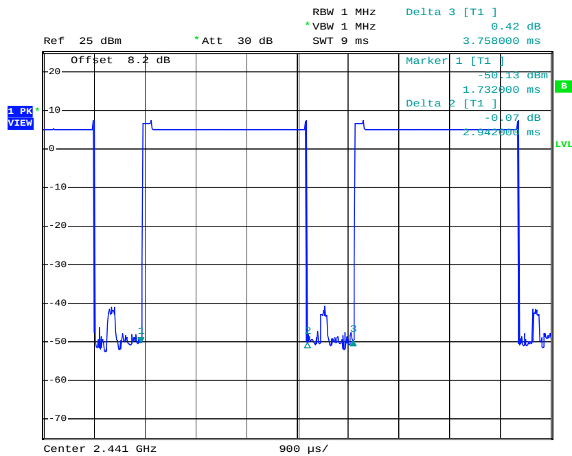
2DH5 Dwell Time (Count Pulses) Plot on Channel 39
