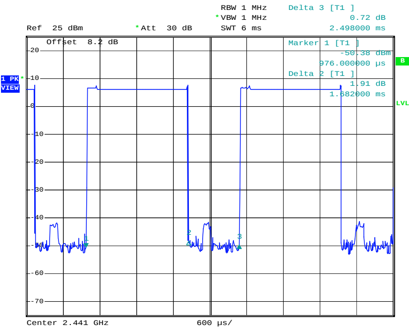
3DH3 Dwell Time (One Pulse) Plot on Channel 39
