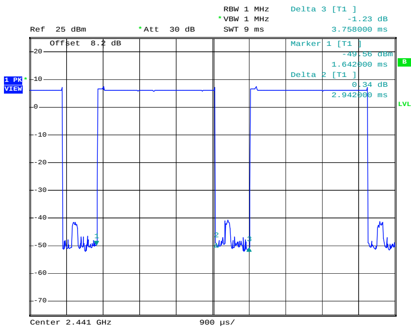
3DH5 Dwell Time (One Pulse) Plot on Channel 39
