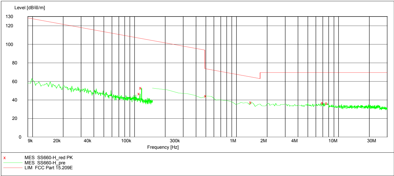
Radiated Emission Plot between 9 kHz ~ 30MHz (Horizontal)
