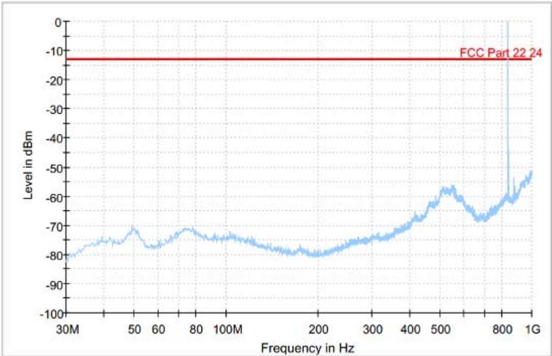
Field Strength of Spurious Radiated 30MHz-1GHz Horizontal
