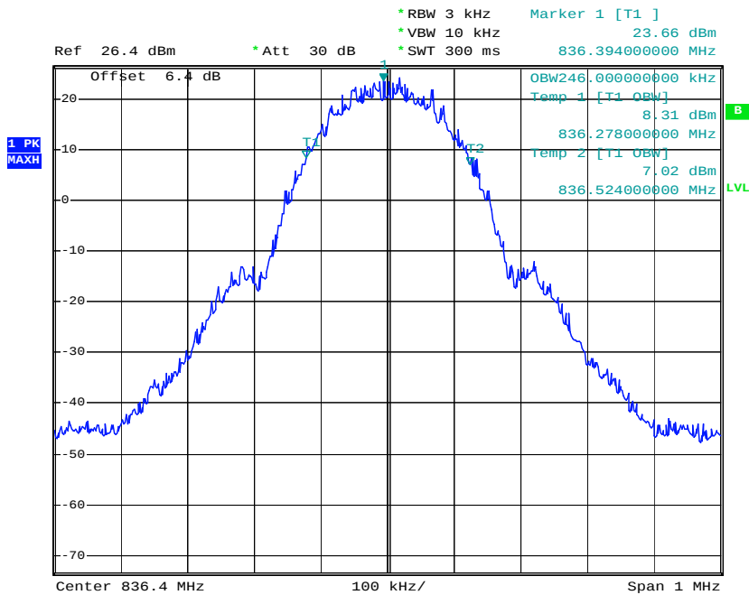
99% Occupied Bandwidth Plot on Channel 189
