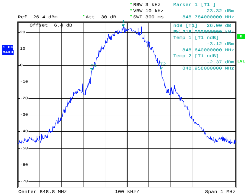
26dB Bandwidth Plot on Channel 251
