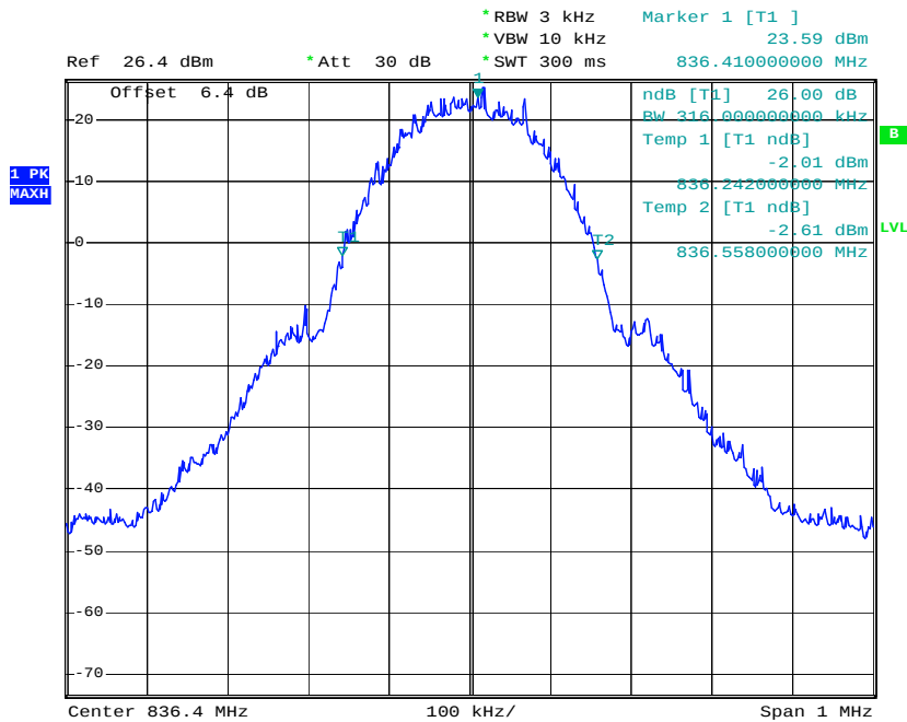
26dB Bandwidth Plot on Channel 189
