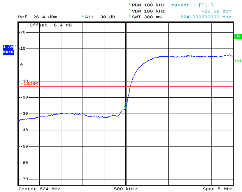
Lower Band Edge Plot on Channel 4132
