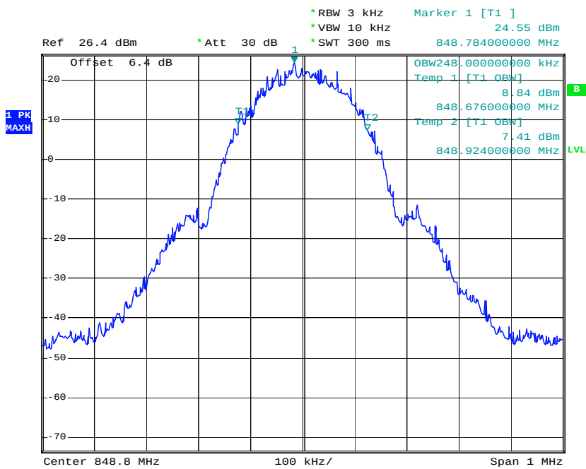
99% Occupied Bandwidth Plot on Channel 251
