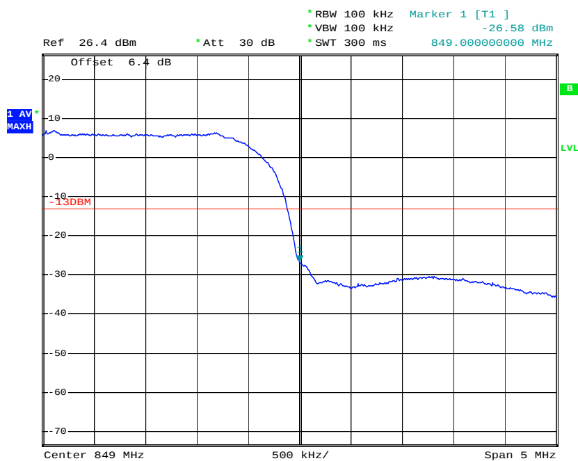
Higher Band Edge Plot on Channel 4233
