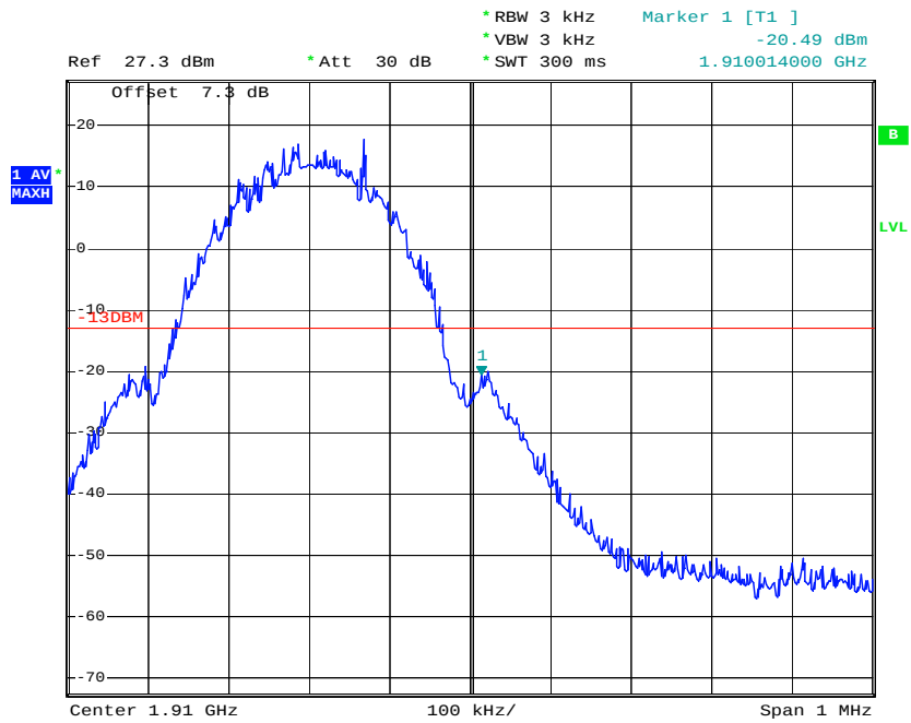
Higher Band Edge Plot on Channel 810
