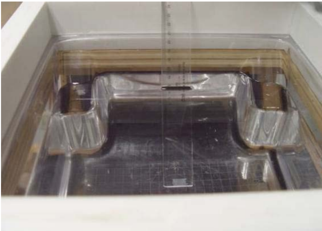
Photo of Liquid Height for Body SAR
