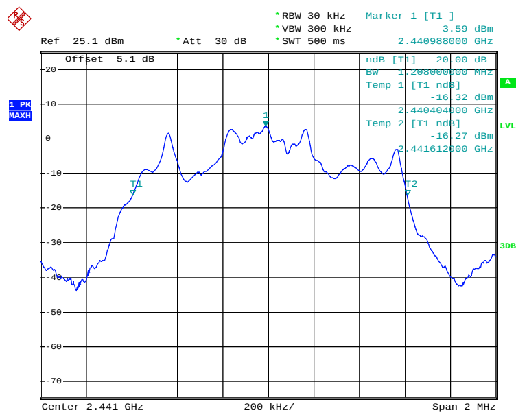
20 dB Bandwidth Plot on Channel 39
