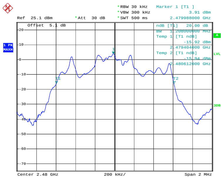
20 dB Bandwidth Plot on Channel 78
