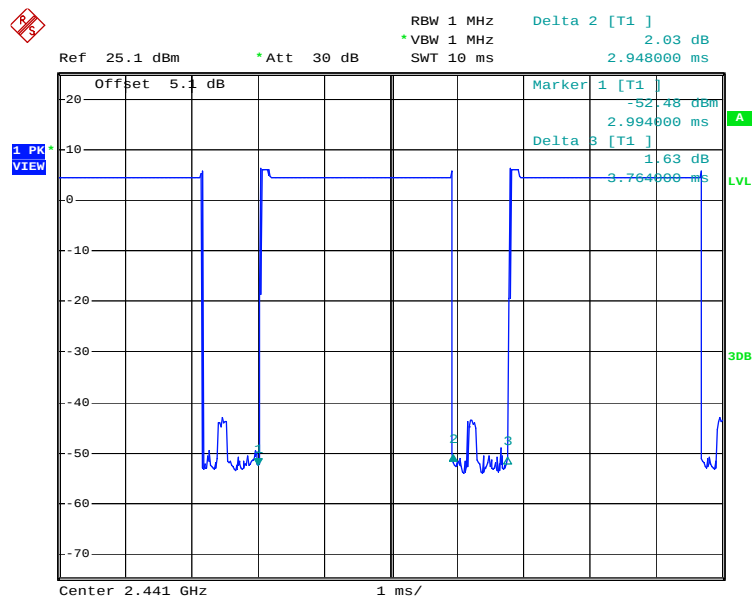
2DH5 Dwell Time (One Pulse) Plot on Channel 39
