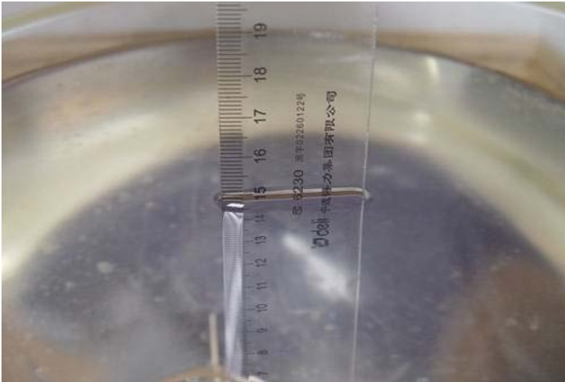
Photo of Liquid Height for Head SAR
