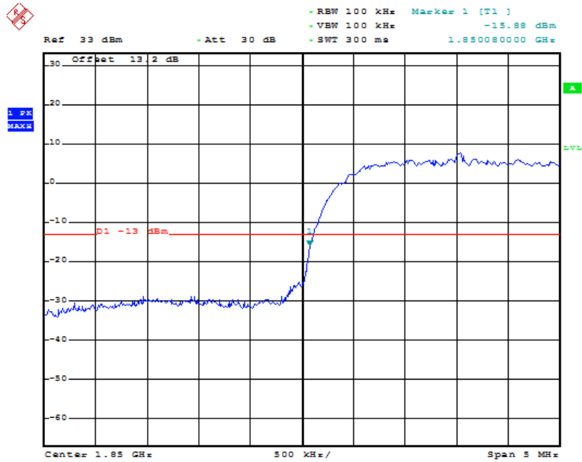
Lower Band Edge Plot on Channel 9262
