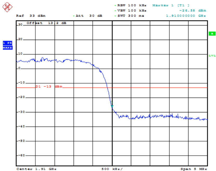
Higher Band Edge Plot on Channel 9538
