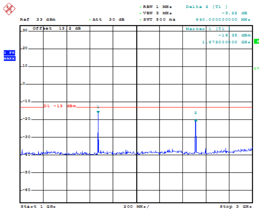
Conducted Emission Plot between 1GHz ~ 3GHz
