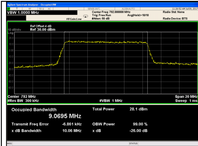
LTE band XIII - Low CH QPSK-10
