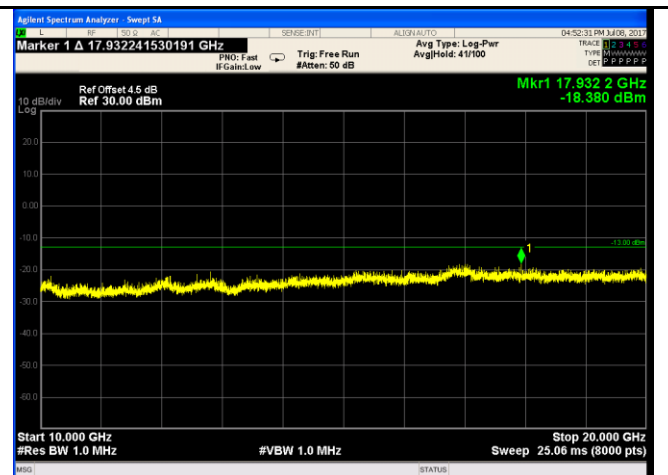
LTE band II Middle Channel-2
