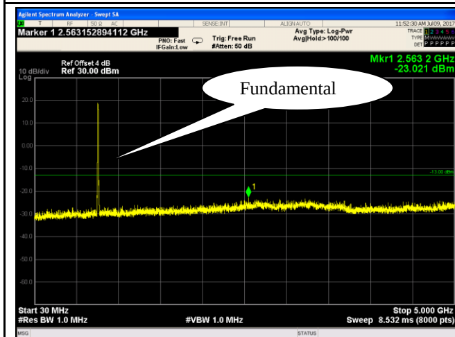
LTE band XIII - High Channel-1
