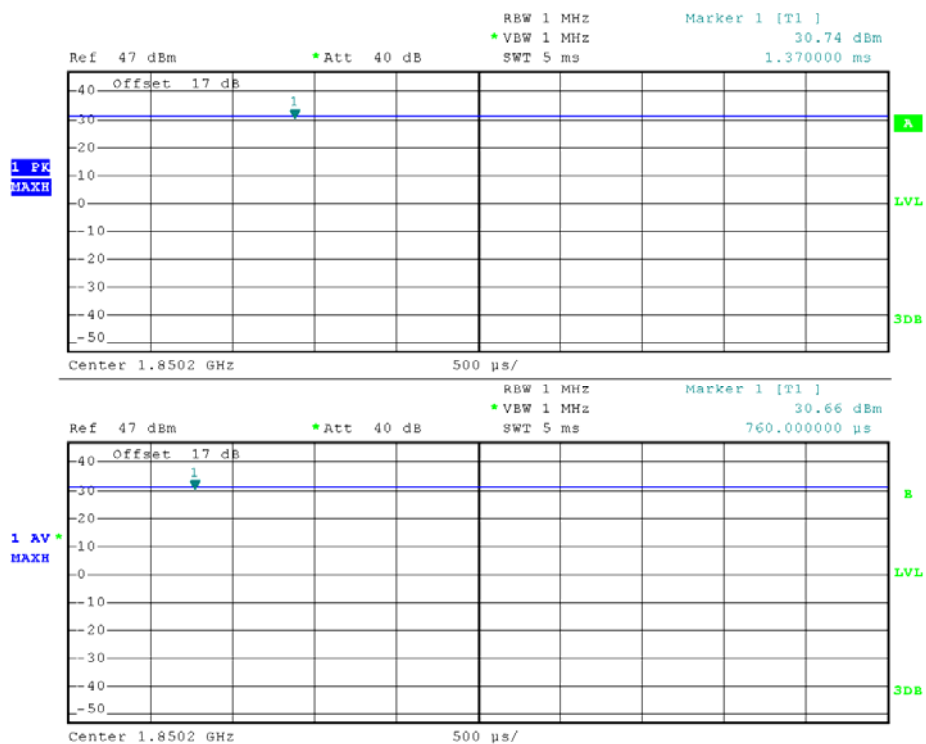
(Plot B1: EDGE 1900 MHz Channel = 512)
