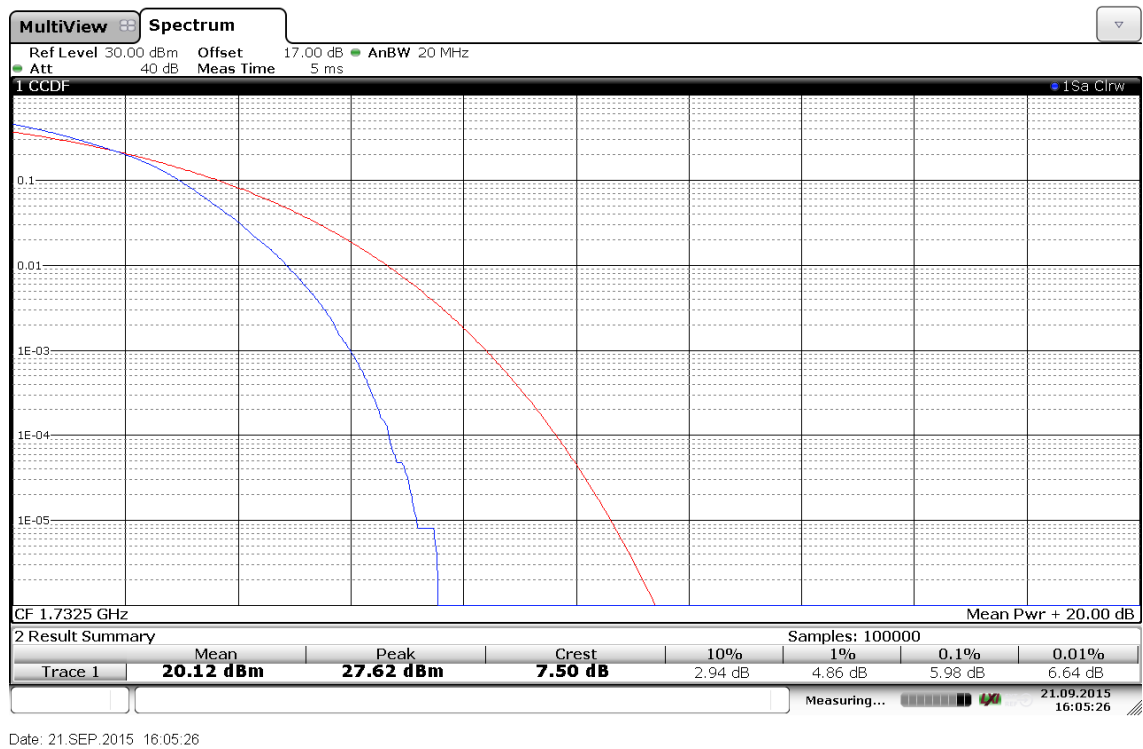
(Plot B4: Band 4/20MHz/16QAM in Ch.20175 100RB Size)
