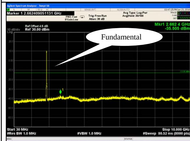
LTE Band 2 Middle Channel-1
