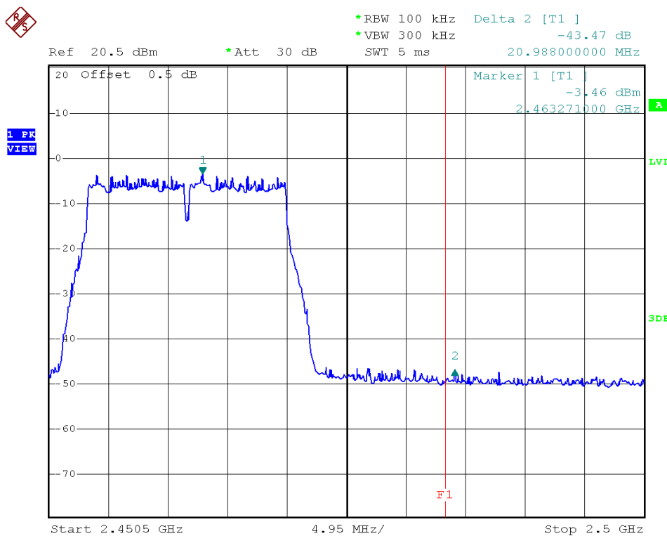
(Plot 2.6 F2: Channel =11 2462MHz @ 802.11g)
