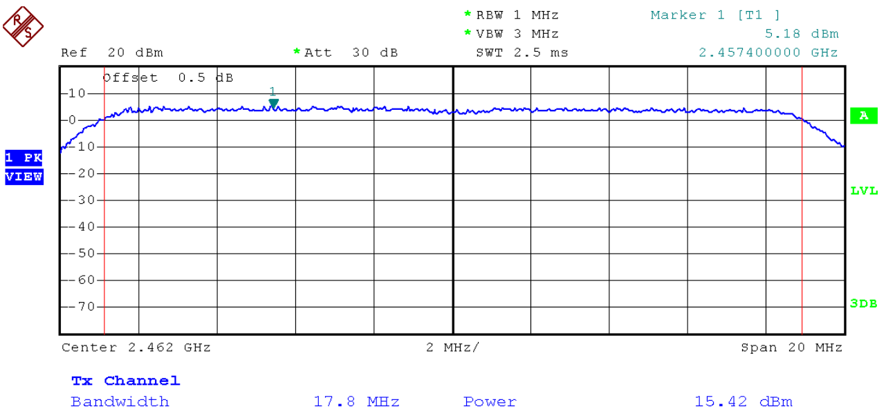
(Plot 2.2 I: Channel 11: 2462MHz @ 802.11n20)
