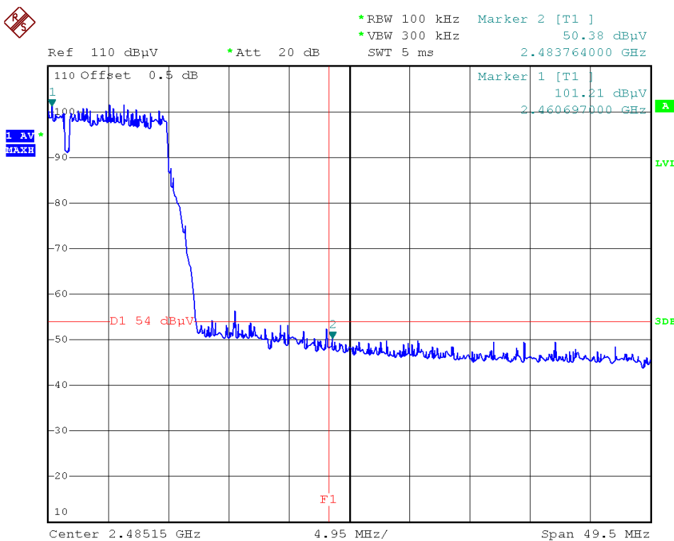
(Plot 2.6 B4: Channel = 11 AVG @ 802.11g)
