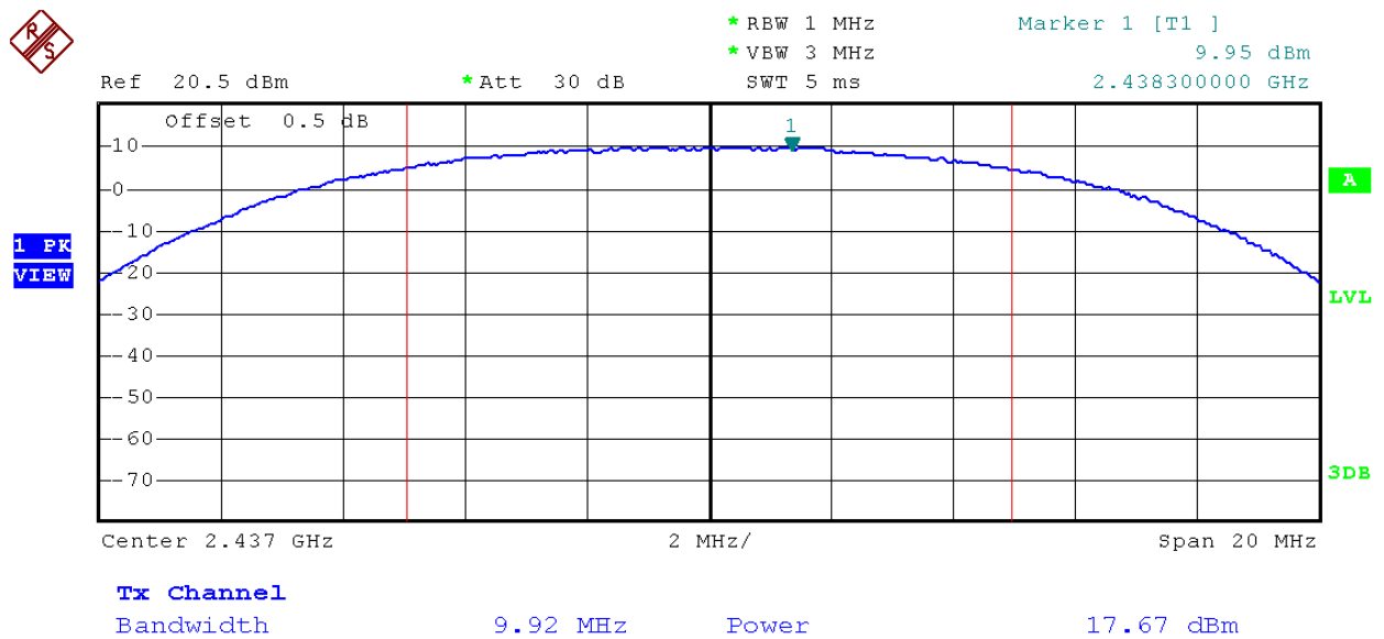
(Plot 2.2 B: Channel 6: 2437MHz @ 802.11b)
