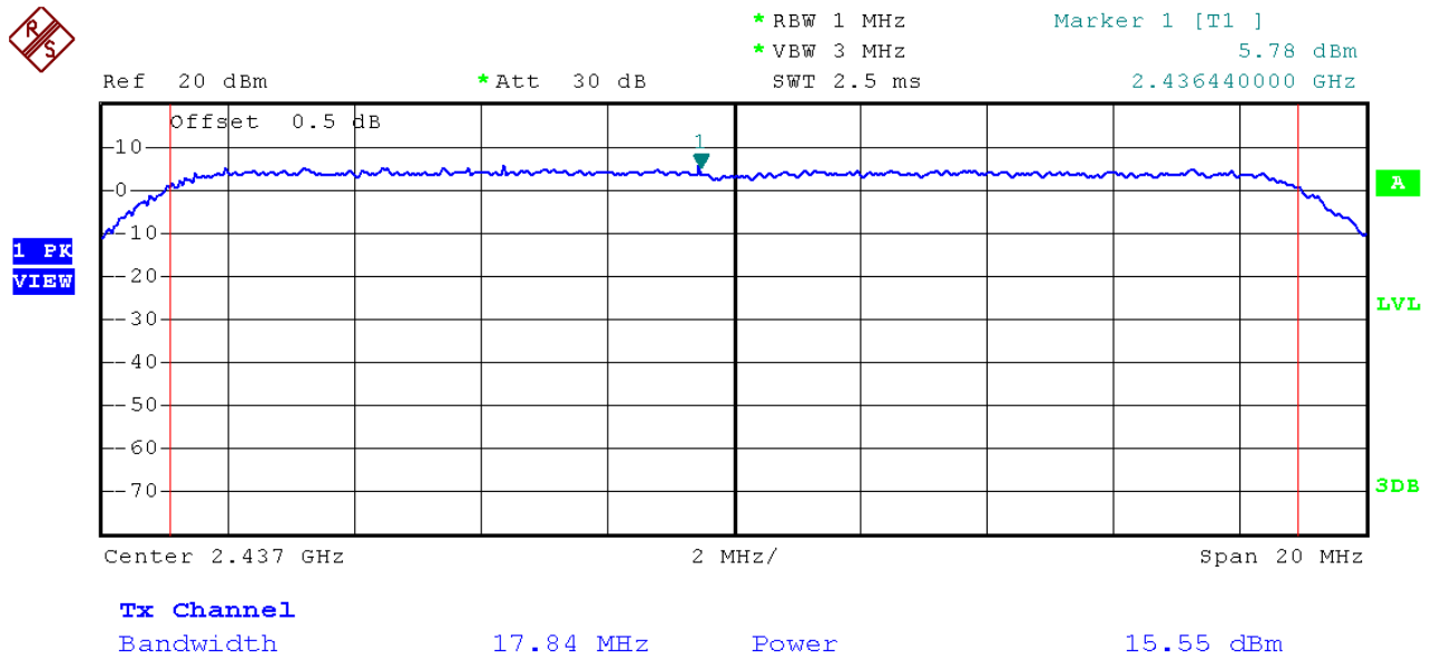
(Plot 2.2 H: Channel 6: 2437MHz @ 802.11n20)
