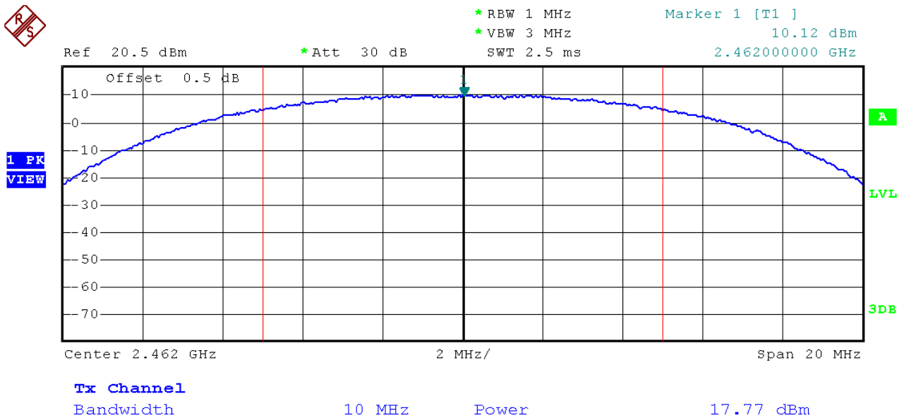
(Plot 2.2 C: Channel 11: 2462MHz @ 802.11b)
