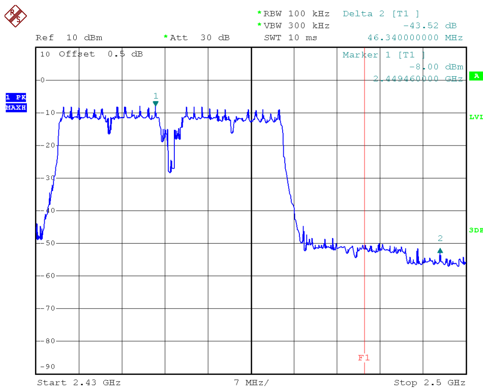
(Plot 2.6 H2: Channel =9 2452MHz @ 802.11n-40)
