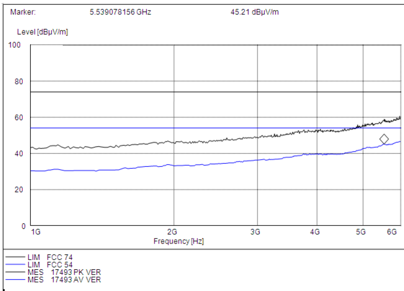
(Plot E: Test Antenna Vertical 1G – 6G)
