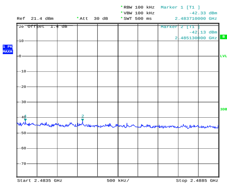
High Band Edge Plot on 802.11g Channel 11
