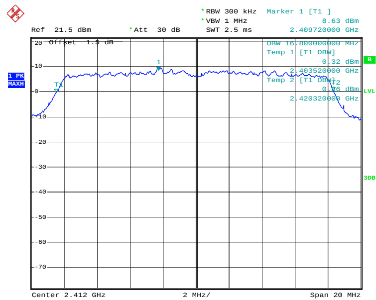
Mode 4 : 99% Occupied Bandwidth Plot on 802.11g Channel 01
