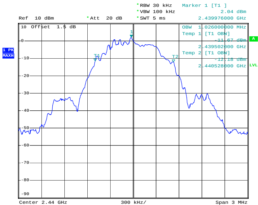
20 dB Bandwidth Plot on Channel 19
