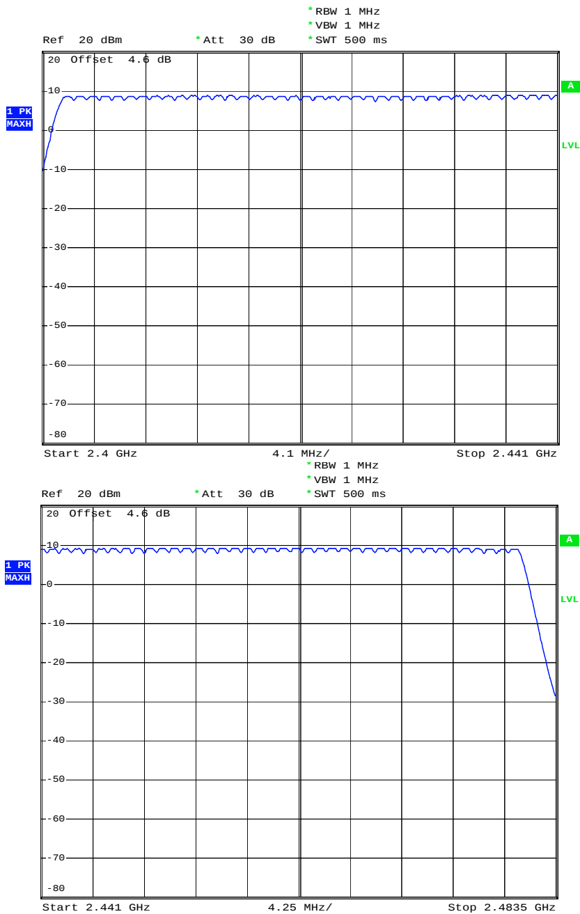
Number of Hopping Channel Plot on Channel 00 - 78
