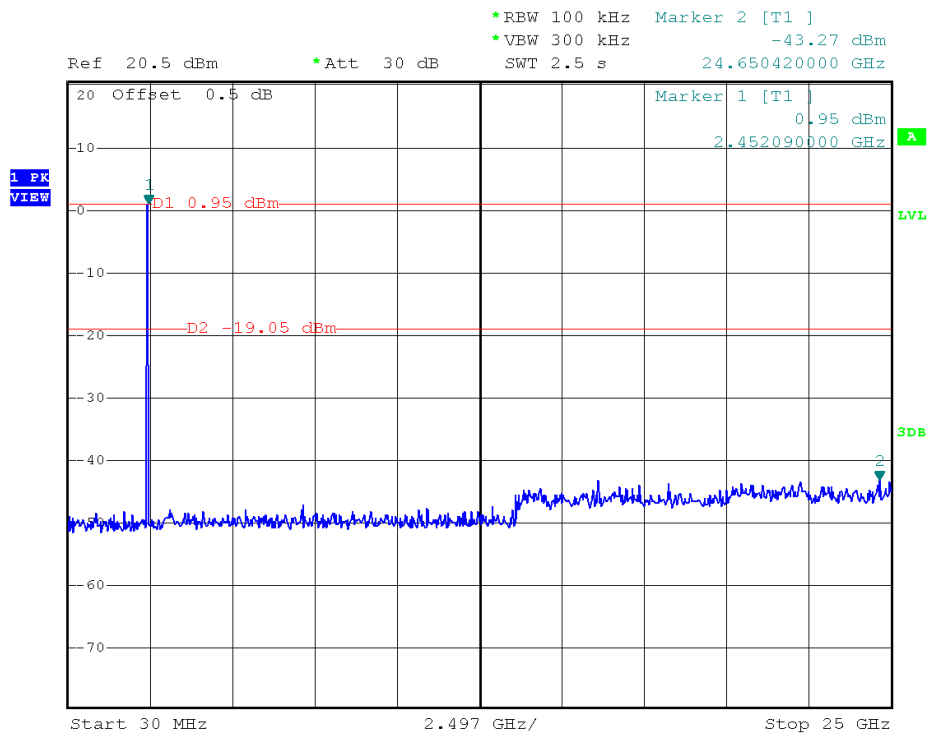
(Plot 2.4 C: Channel = 11, 30MHz to 25GHz@ 802.11b)
