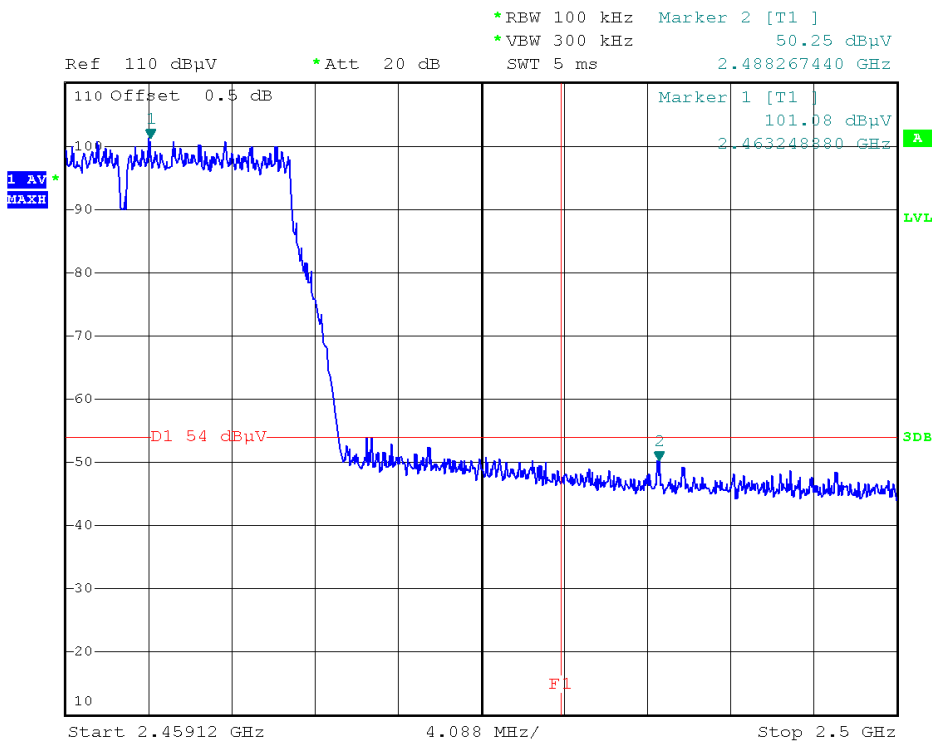
(Plot 2.6 B4: Channel = 11 AVG @ 802.11g)
