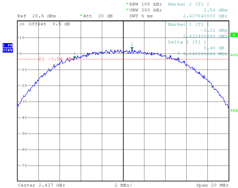
(Plot 2.3 B: Channel 6: 2437 MHz @ 802.11b)
