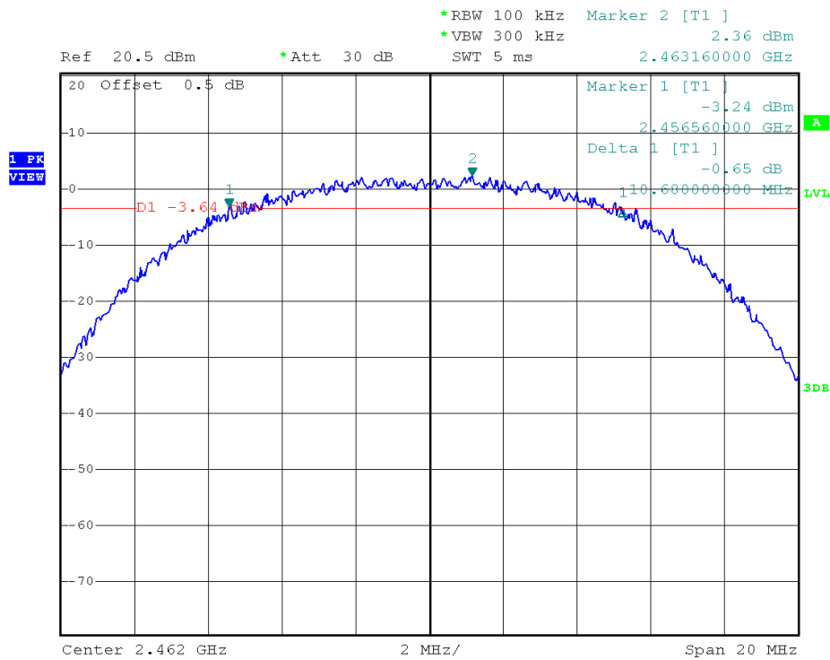
(Plot 2.3 C: Channel 11: 2462MHz @ 802.11b)
