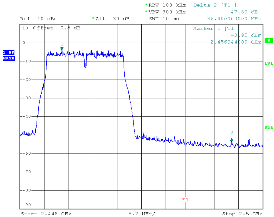
(Plot 2.6 F2: Channel =11 2462MHz @ 802.11g)
