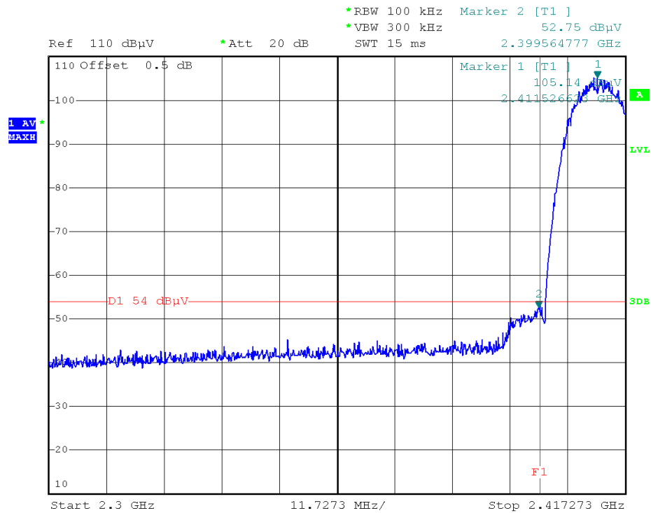
(Plot 2.6 A2: Channel = 1 AVG @ 802.11b)
