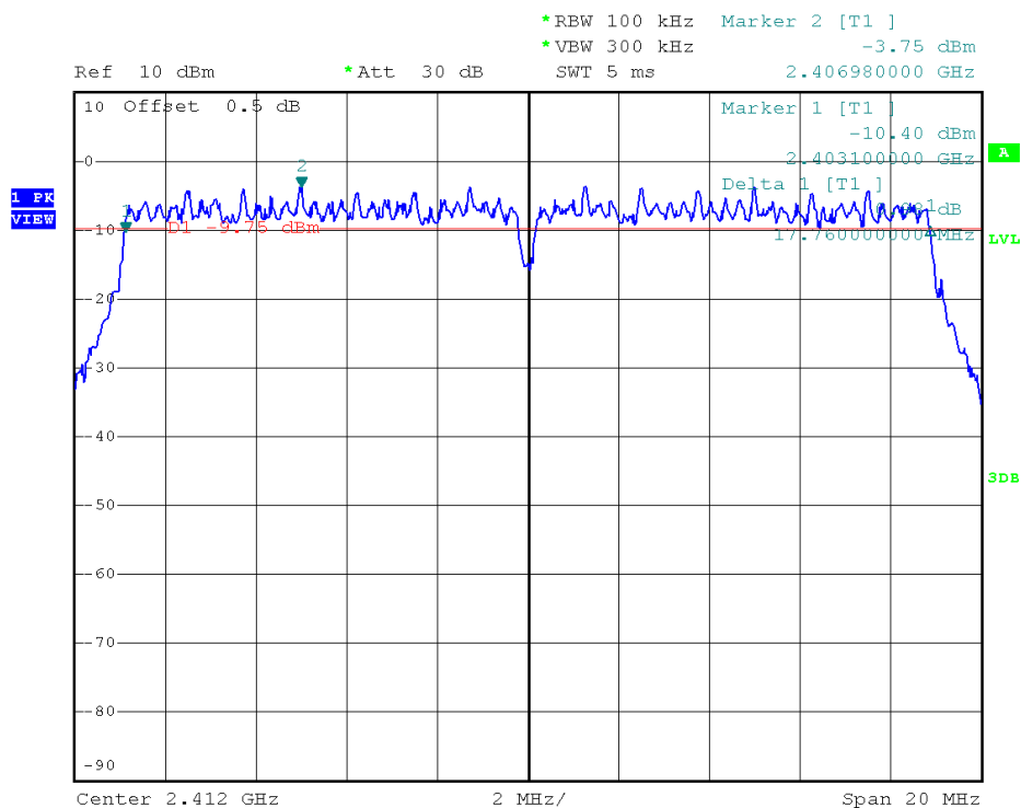
(Plot 2.3 G: Channel 1: 2412MHz @ 802.11n-20)
