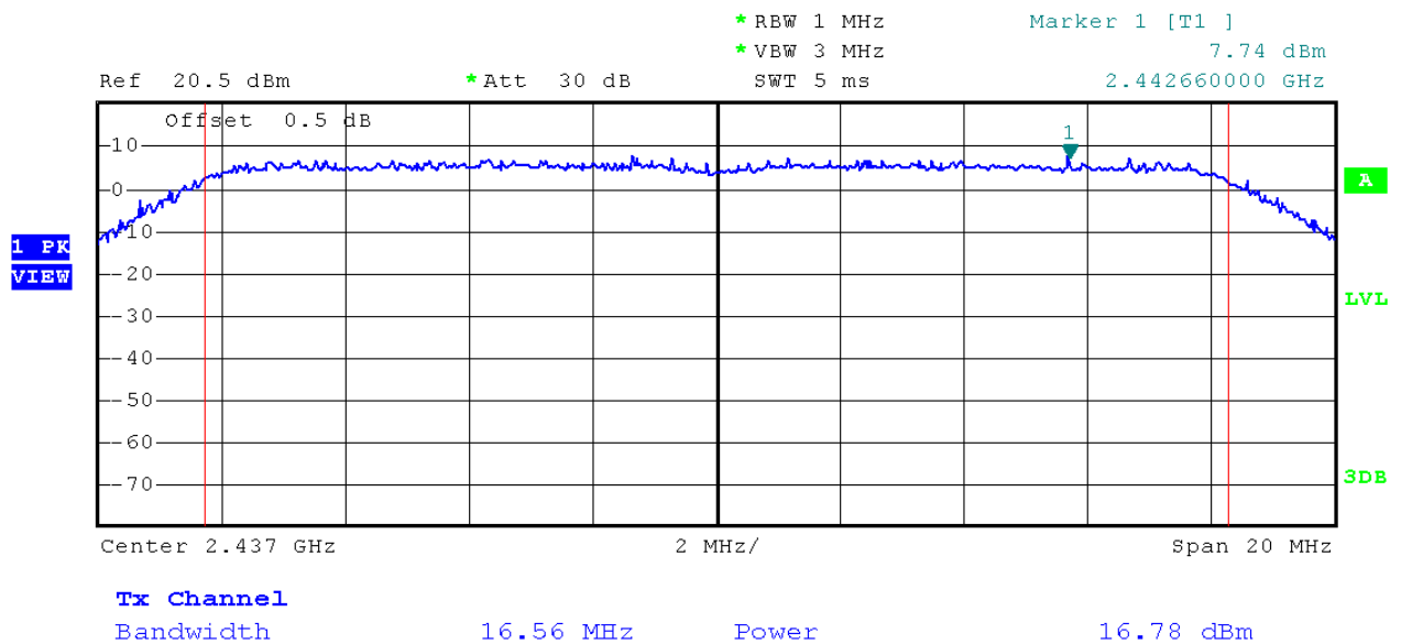
(Plot 2.2 E: Channel 6: 2437MHz @ 802.11g)
