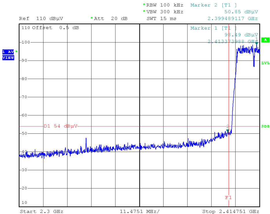
(Plot 2.6 B2: Channel = 1 AVG @ 802.11g)
