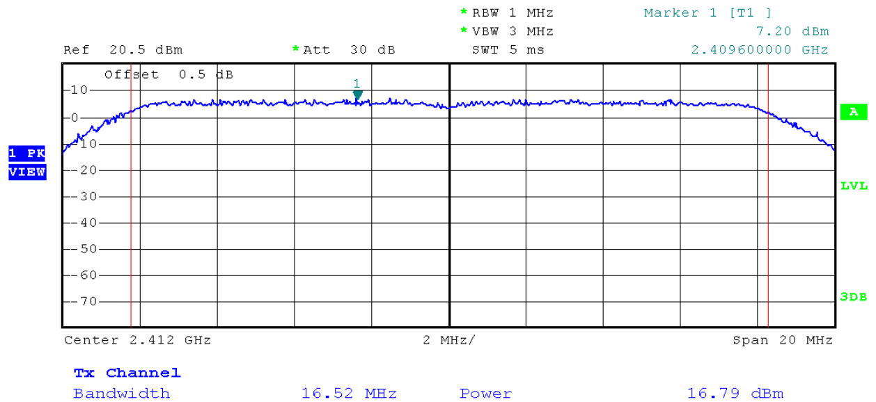
(Plot 2.2 D: Channel 1: 2412MHz @ 802.11g)
