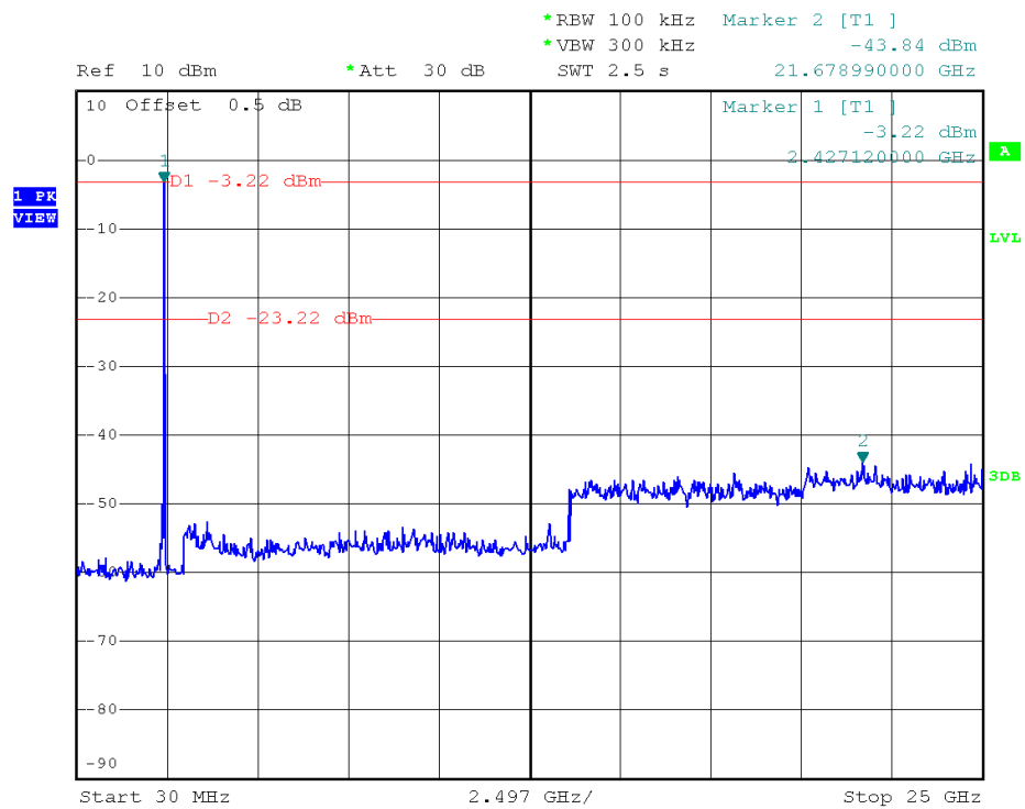
(Plot 2.4 E: Channel = 6, 30MHz to 25GHz@ 802.11g)
