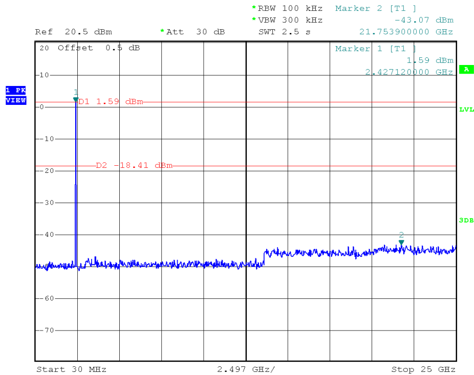
(Plot 2.4 B: Channel = 6, 30MHz to 25GHz@ 802.11b)
