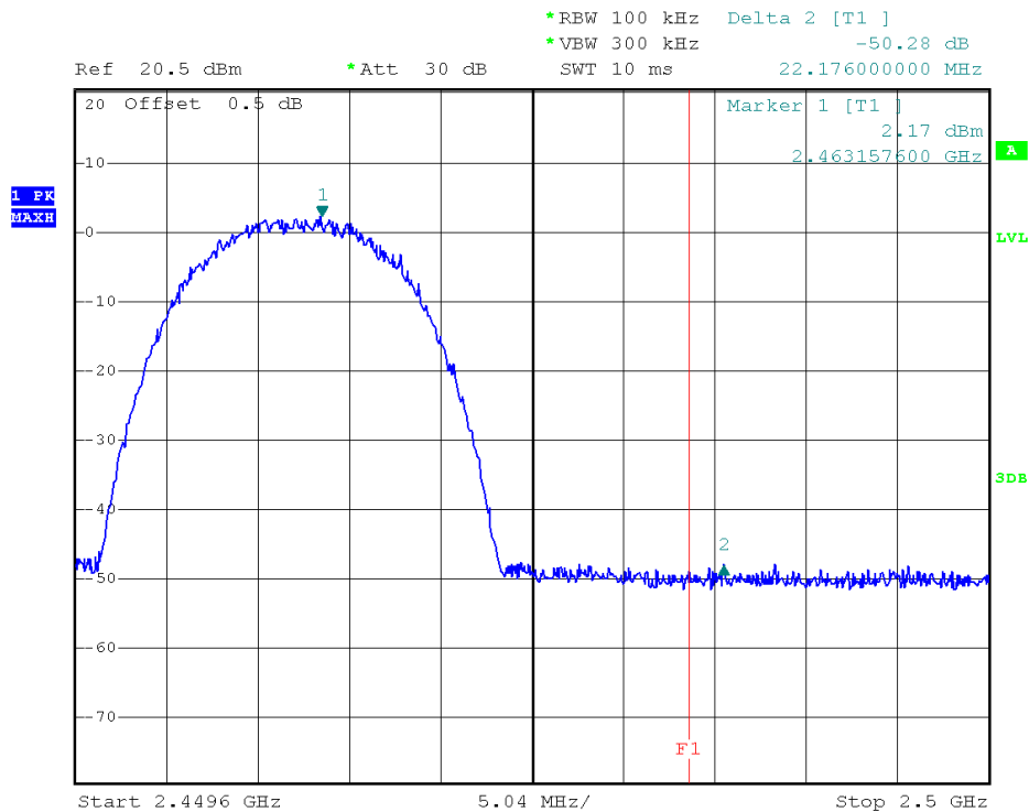
(Plot 2.6 E2: Channel =11 2462MHz @ 802.11b)
