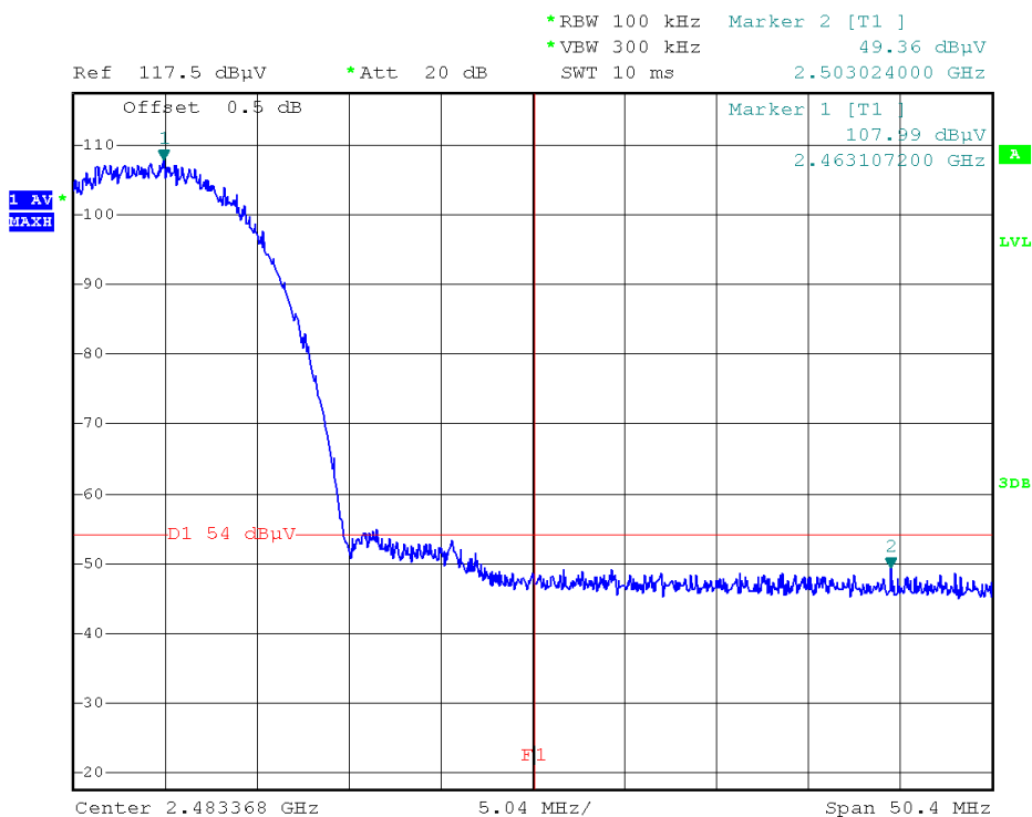
(Plot 2.6 A4: Channel = 11 AVG @ 802.11b)
