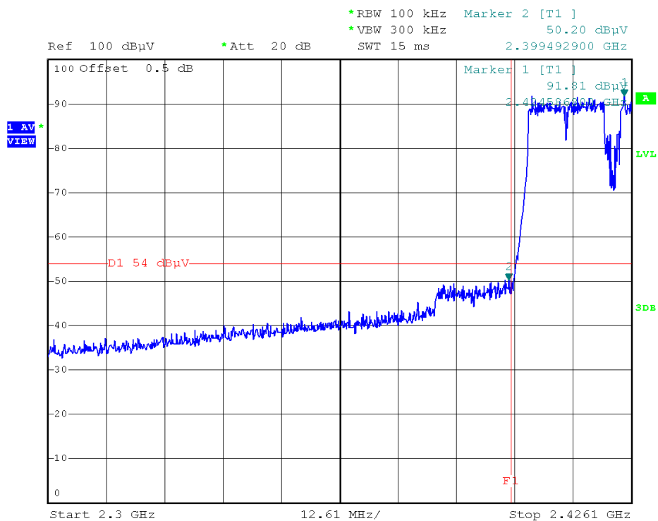
(Plot 2.6 D2: Channel = 3 AVG @ 802.11n-40)
