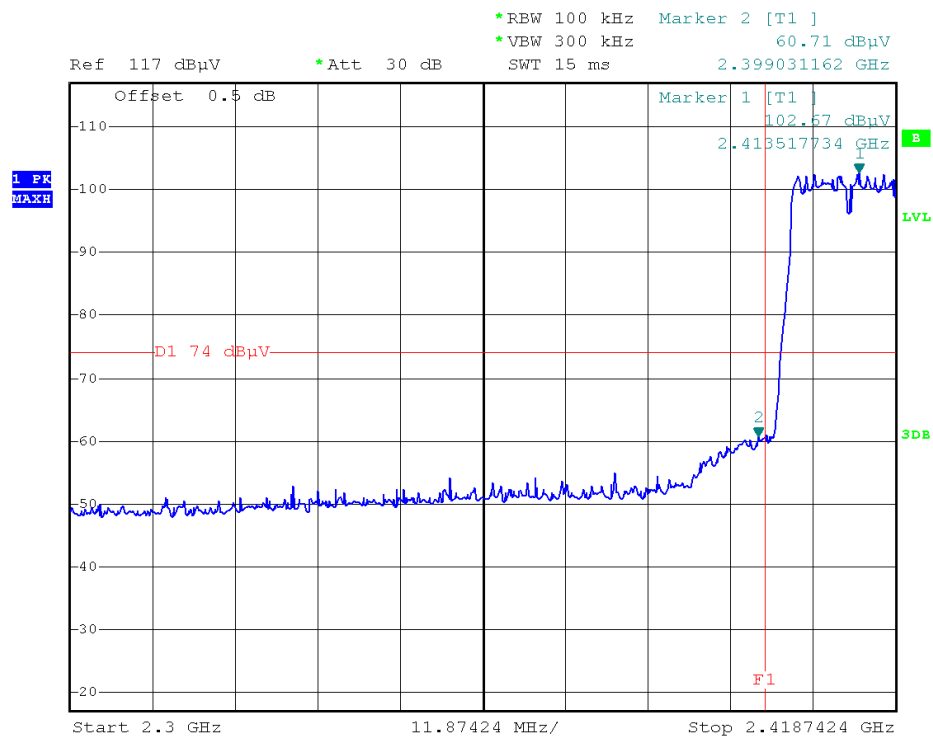
(Plot 2.6 B1: Channel = 1 Peak @ 802.11g)
