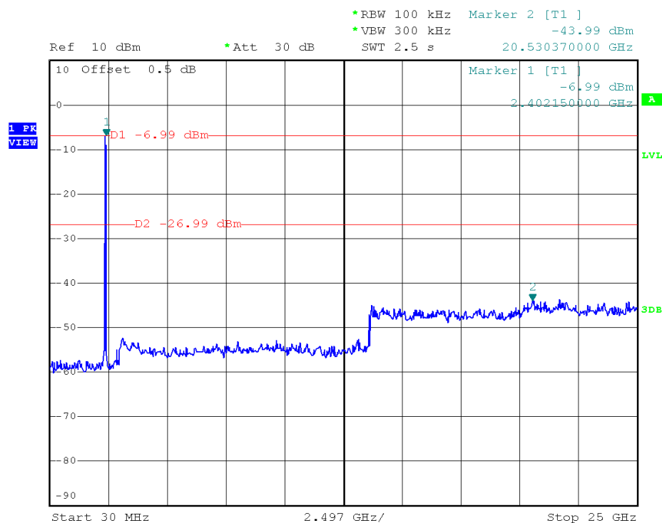
(Plot 2.4 J: Channel = 3, 30MHz to 25GHz@ 802.11n-40)
