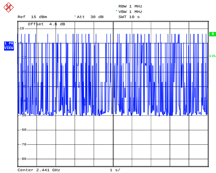
3DH3 Dwell Time (Count Pulses) Plot on Channel 39
