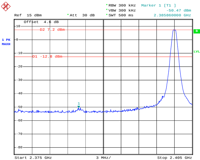
Low Band Edge Plot on Channel 00
