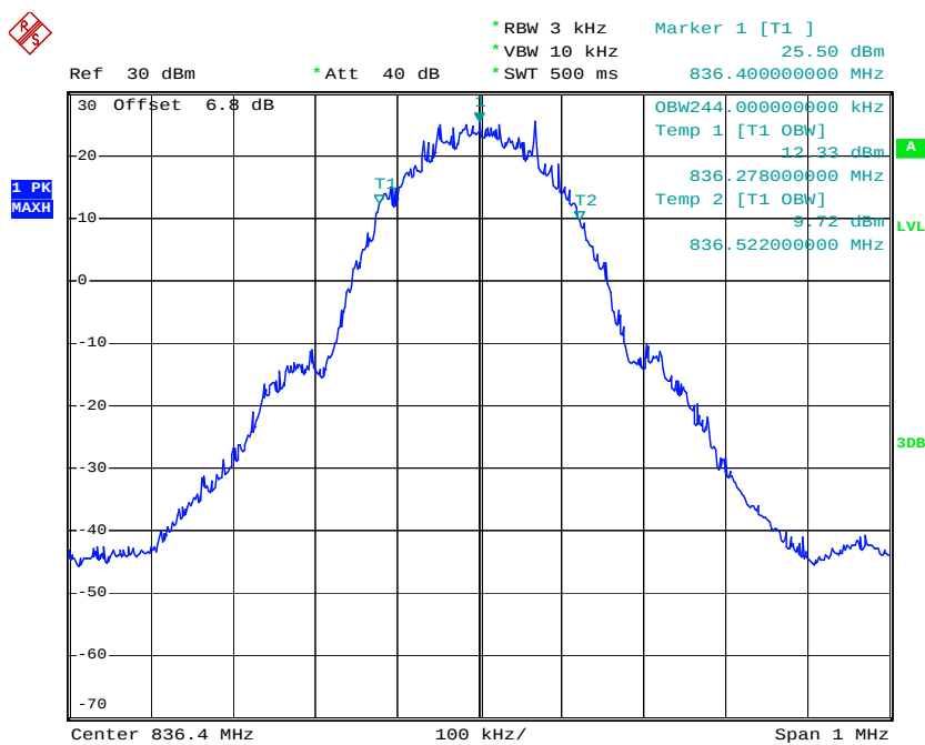
26dB Bandwidth Plot on Channel 189
