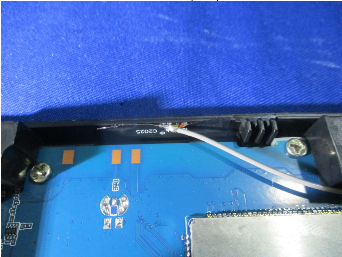
WWAN Inside Main Antenna
