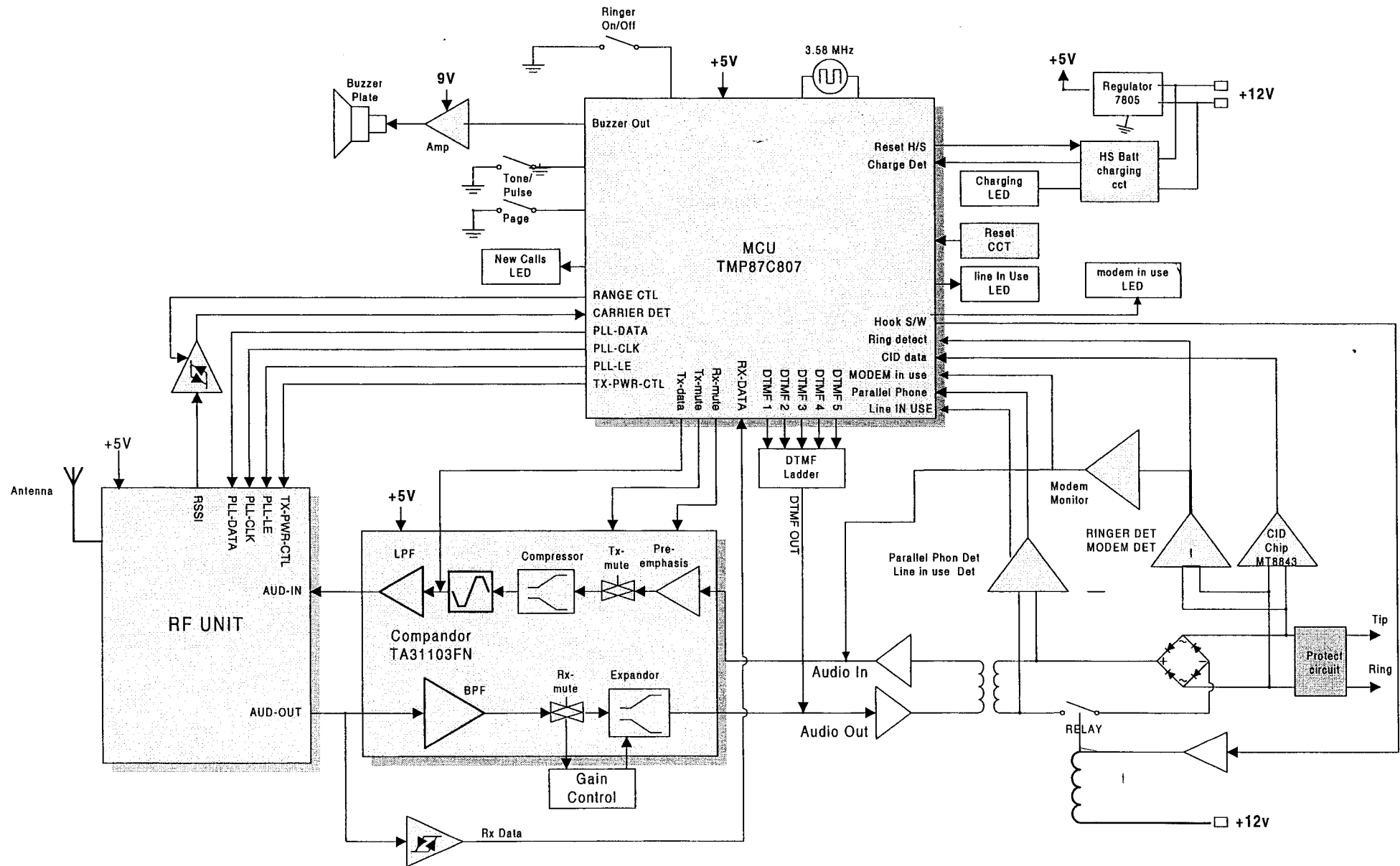
CP-750 Base Block Diagram
