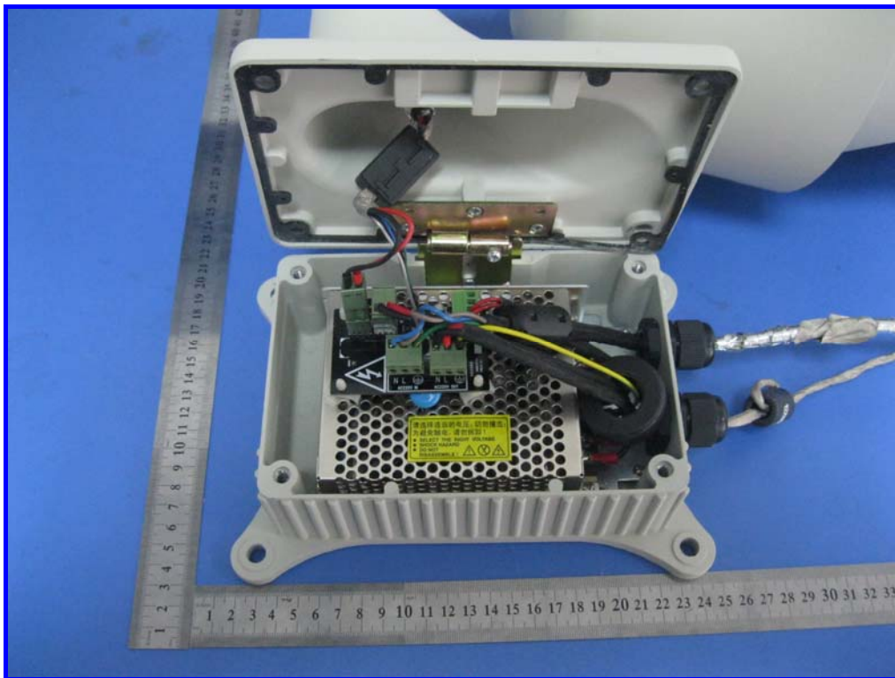
Photo #1 EUT-Uncovered View
