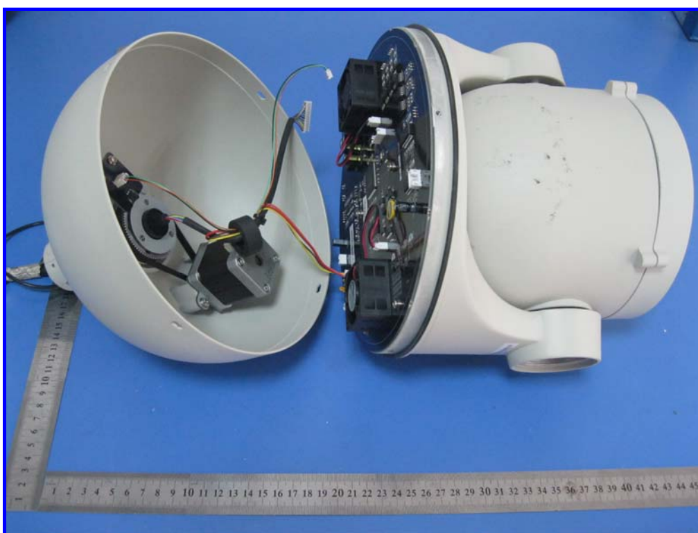
Photo #8 Front of view- Motherboard internal
