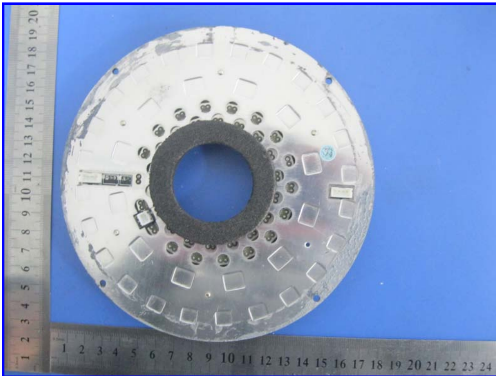
Photo #15 Rear of view- LED board
