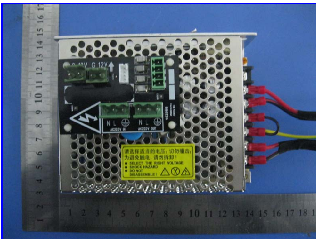
Photo #2 Front of view- Power box
