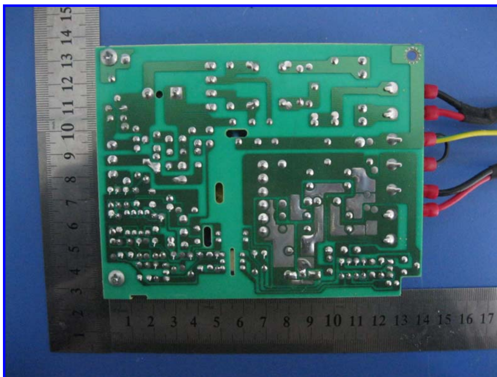
Photo #6 Rear of view- Power board
