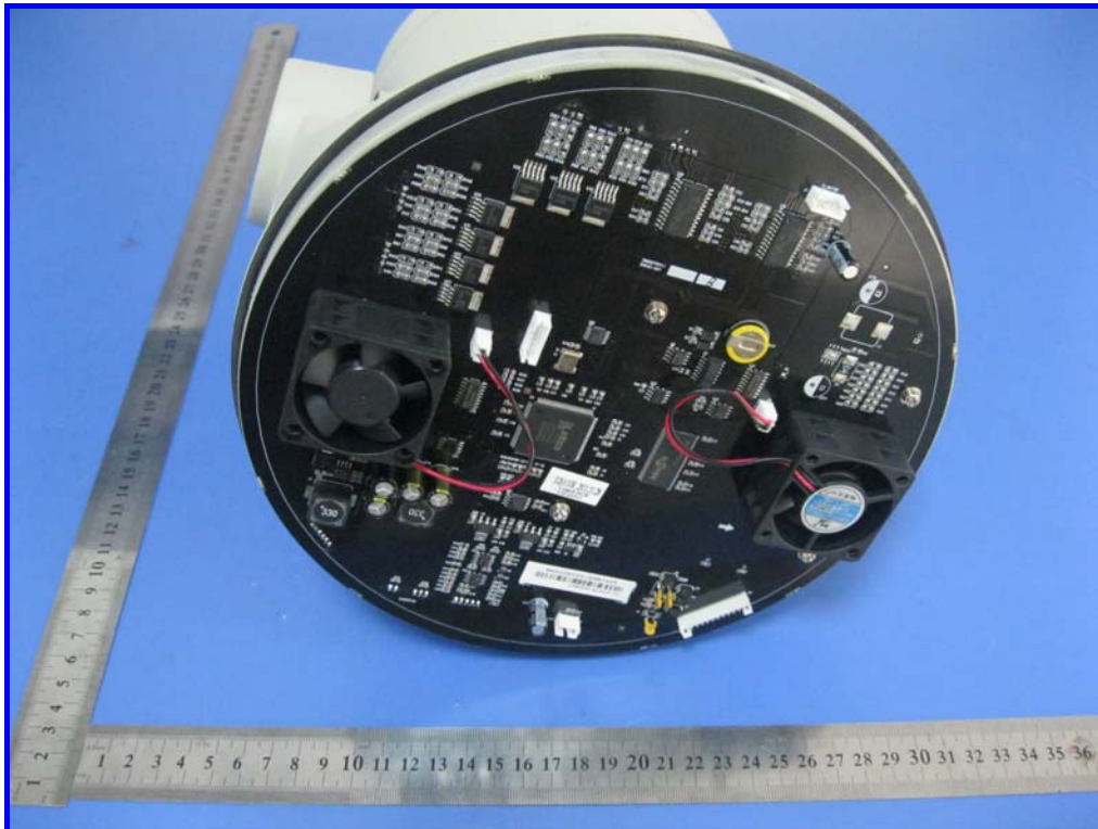
Photo #10 Front of view- motherboard
