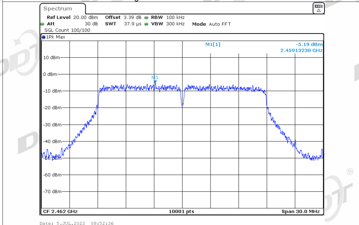
Band Edge NVNT n20 2462MHz Ant1 Emission
