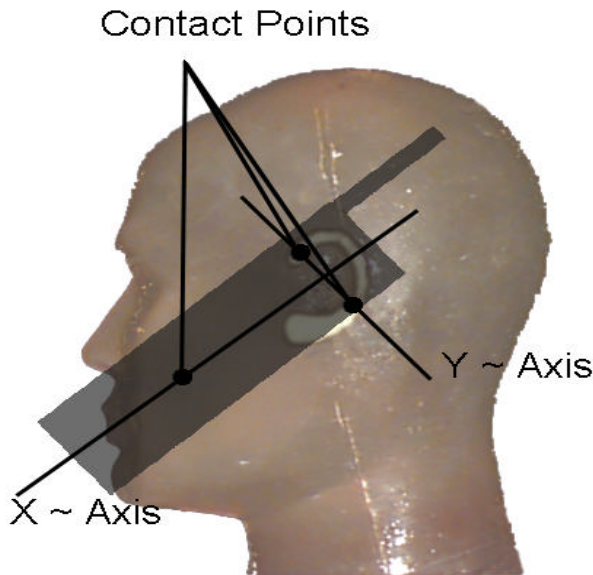
Figure 8. Diagram showing Typical Alignment & Contact Points
