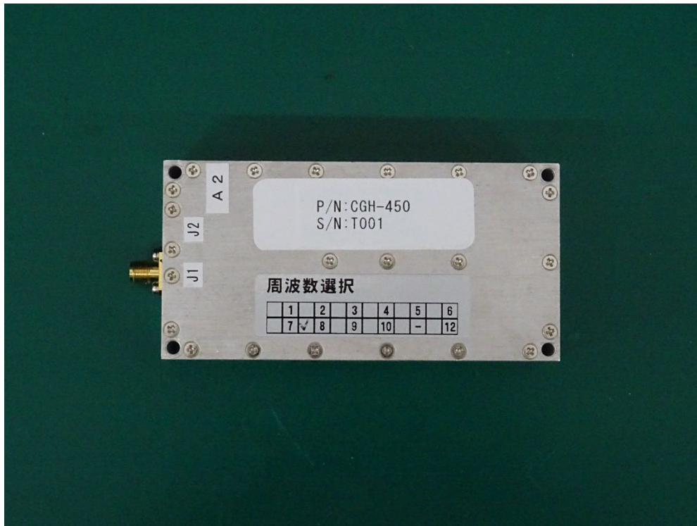
Oscillator Module (1 st Local/CGH-450) Top View
