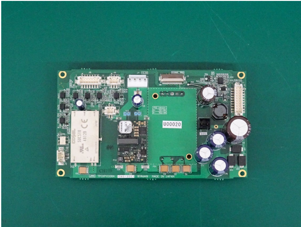
PS I/F Circuit (CBD-2027) Top View
