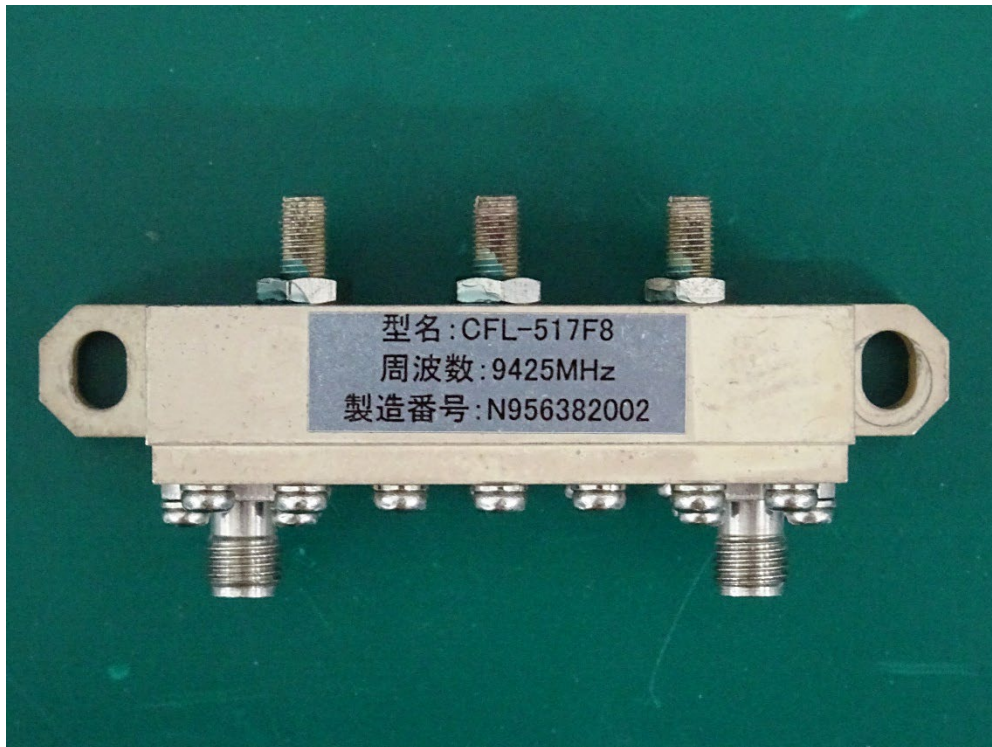
Band Pass Filter (TX / CFL-517F8)
