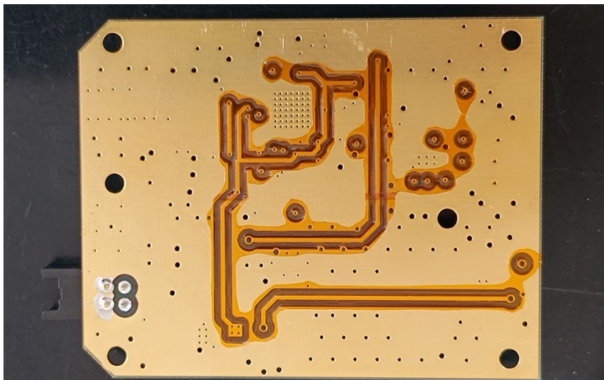
Oscillator Module (2 nd Local/CGH-382A) Oscillator Circuit Bottom View
