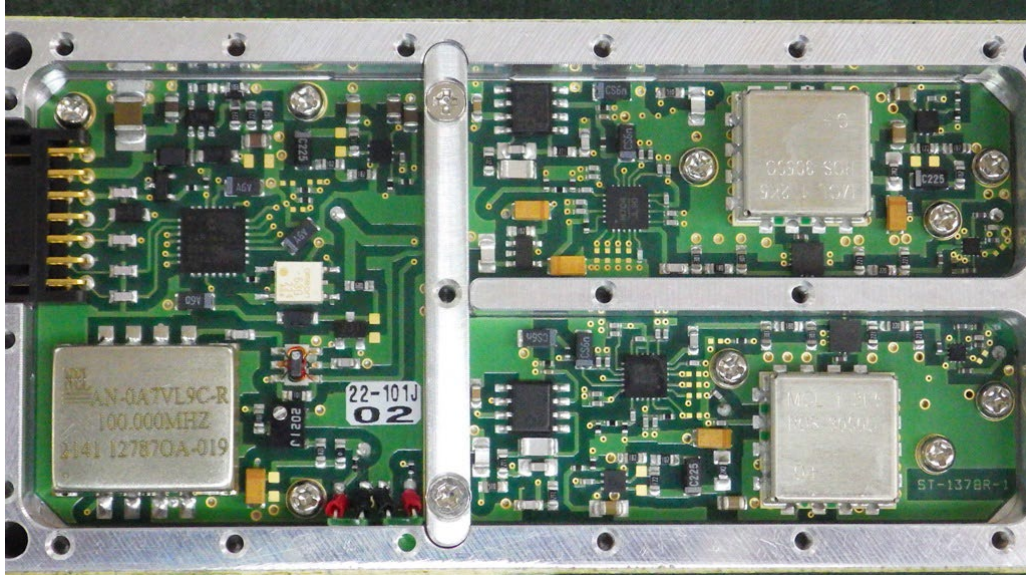
Oscillator Module (1 st Local/CGH-450) Oscillator Circuit Top View
