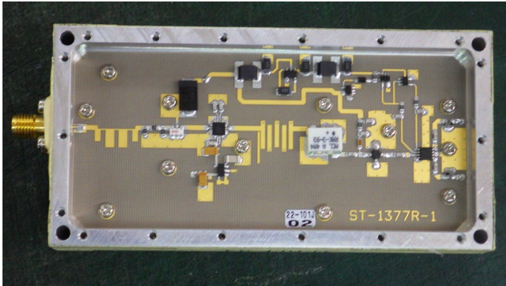
Oscillator Module (1 st Local/CGH-450) RF Circuit Top View
