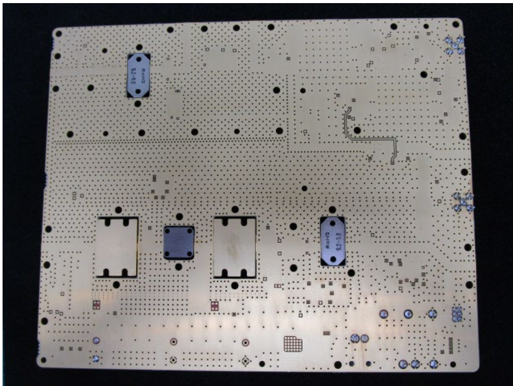
TRX Module (CMN-821H) Circuit View (GND Plane side)
