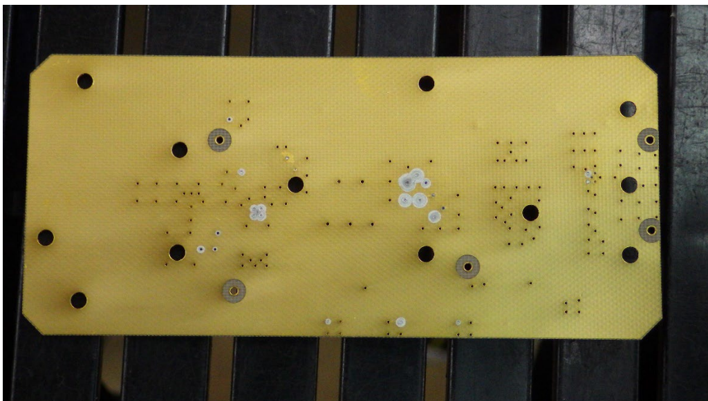
Oscillator Module (1 st Local/CGH-450) RF Circuit Bottom View
