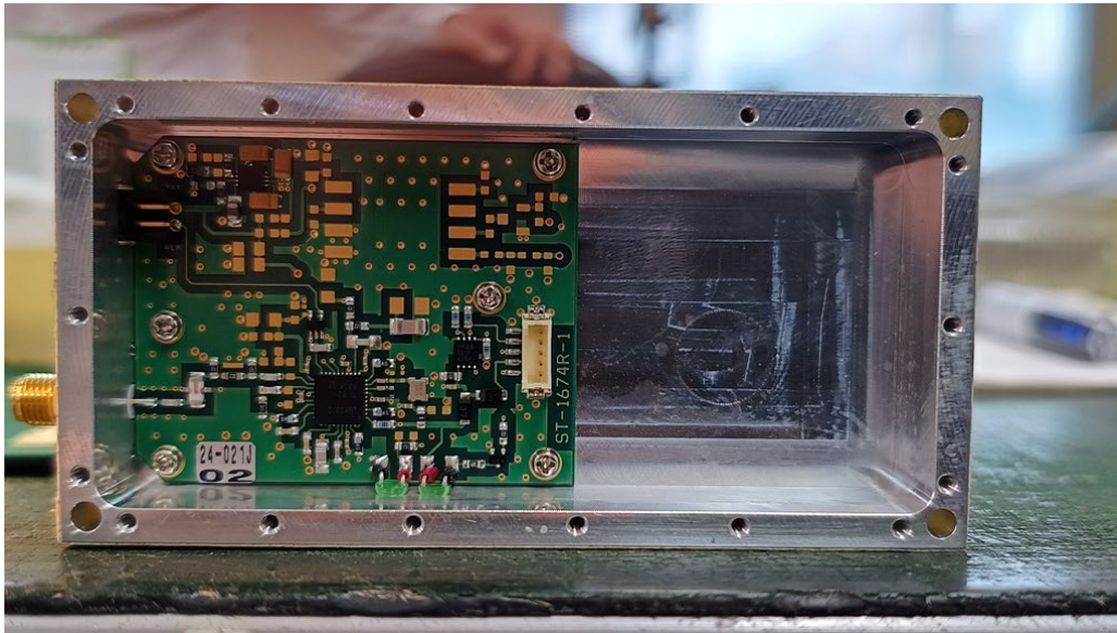
Oscillator Module (2 nd Local/CGH-382A) Oscillator Circuit Top View
