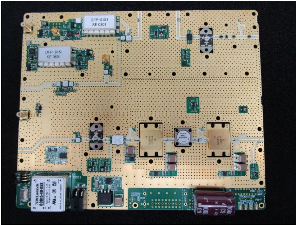
TRX Module (CMN-821H) Circuit View (Parts side)
