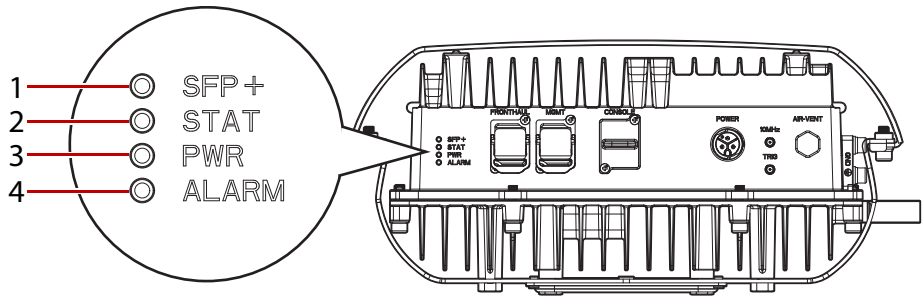
Figure 1-4. System Indicators
