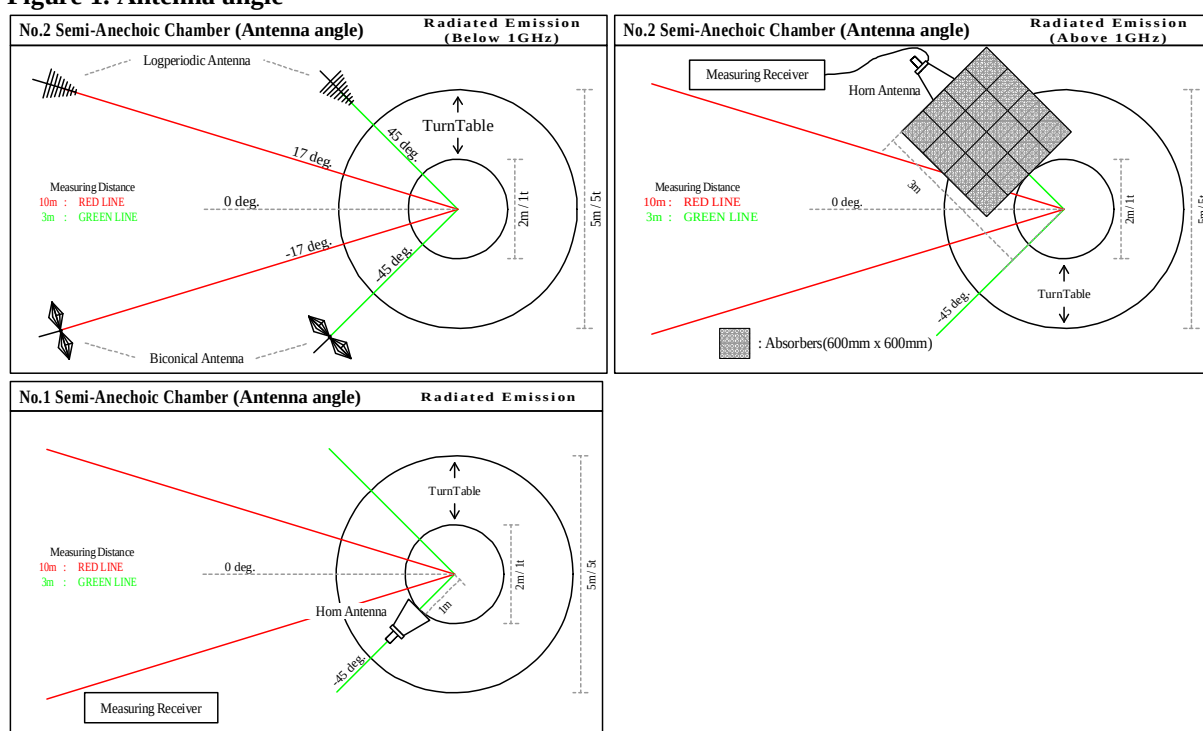
Figure 1. Antenna angle
