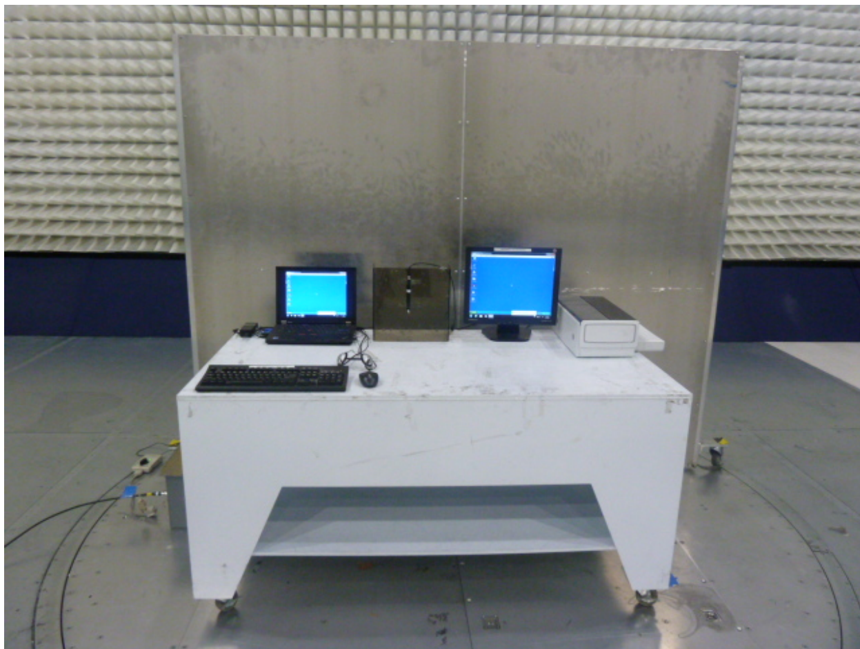
Test Setup Photographs AC Line conducted Emission
