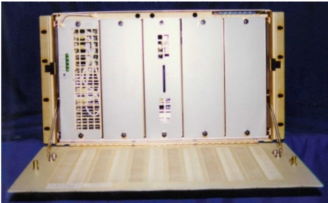
4.3.15 Front view, Intermediate Broadband Amplifier tray (open front door)
