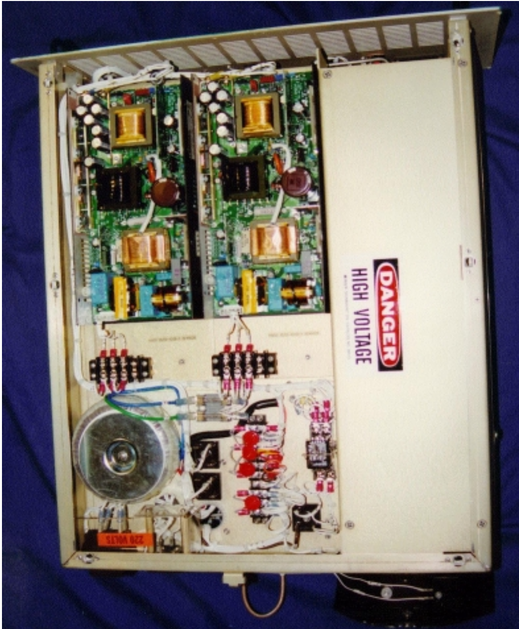
4.3.13 Bottom view, Broadband Translator tray (Switching Power Supplies)
