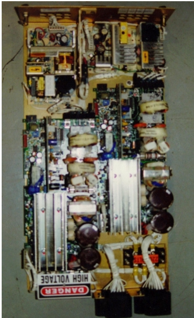
4.3.23 Top view, Broadband Amplifier tray (Power Supply Module)
