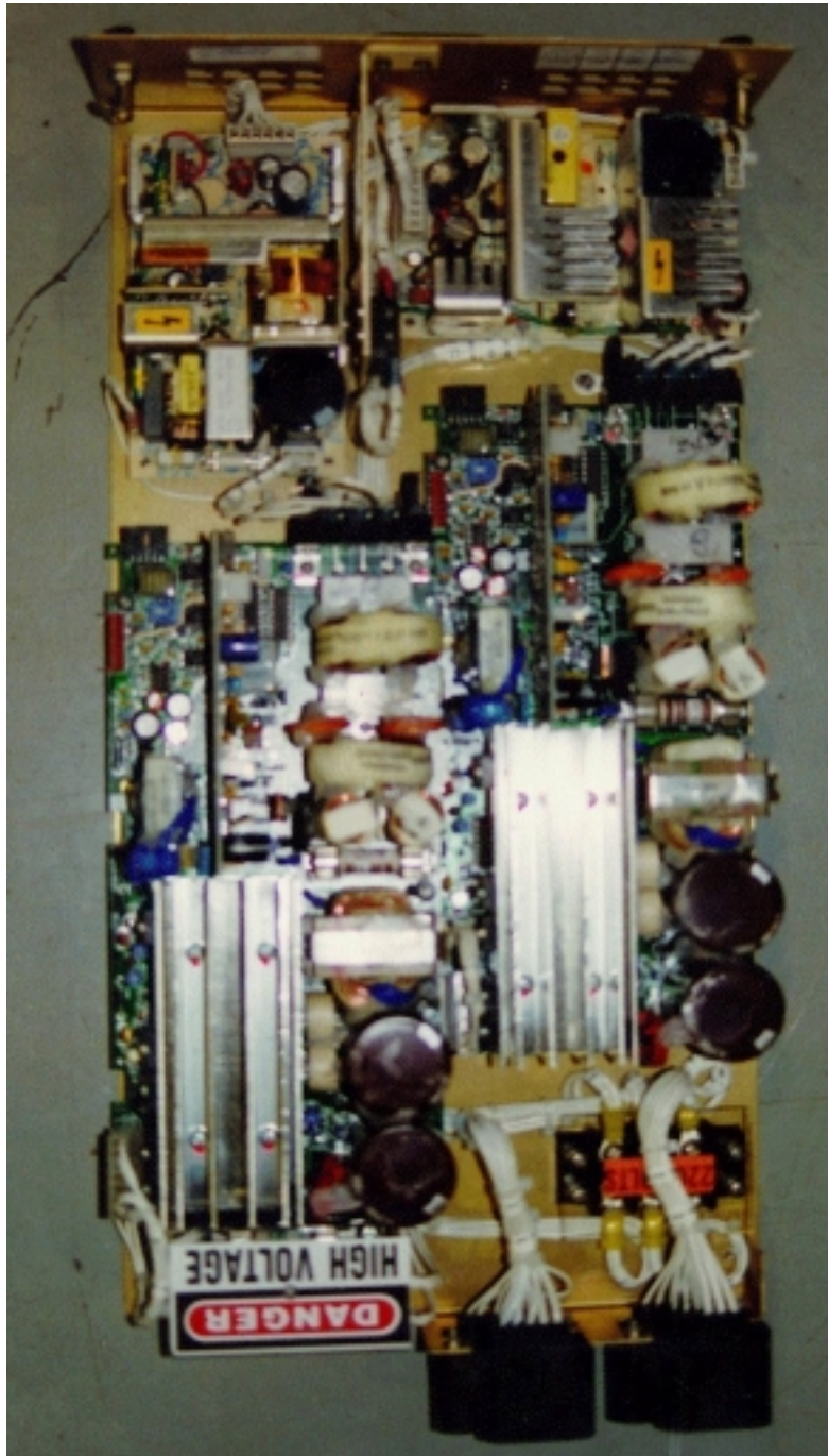
4.3.18 Top view, Intermediate Broadband Amplifier tray (Power Supply)
