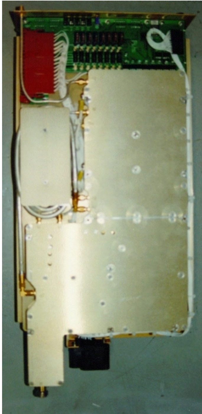
4.3.17 Top view, Intermediate Broadband Amplifier tray (Power Amplifier Module)
