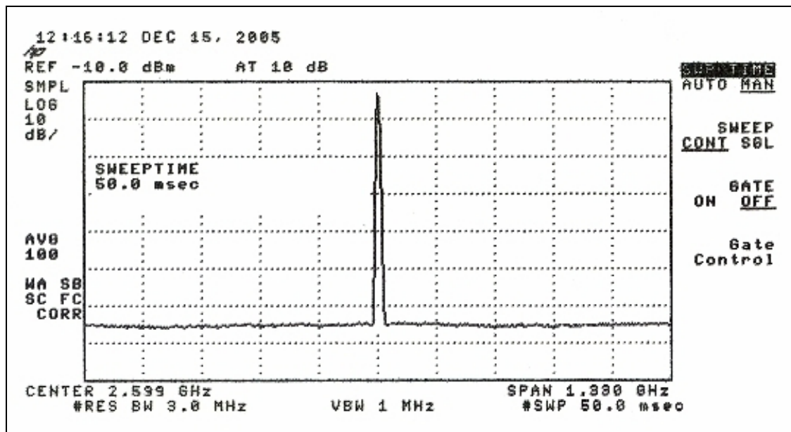
Figure 4-7. Products Above the -62 dB Noise Floor of the Spectrum Analyzer (1.330 GHz Span)
