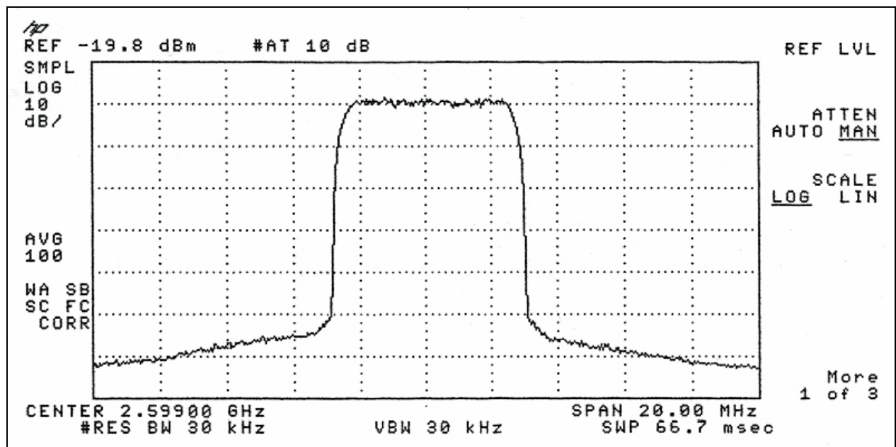
Figure 4-5. Channel Occupied Bandwidth
