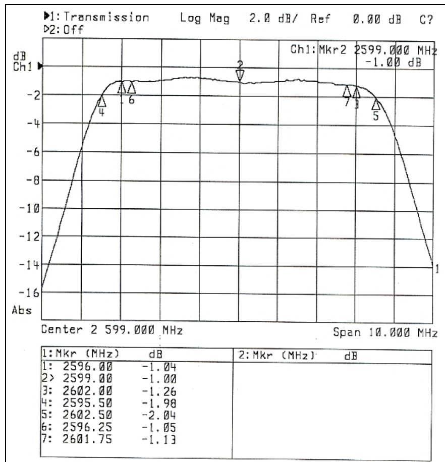
Figure 4-9. Conducted Spurious Emissions (Filter response of channel filter)
