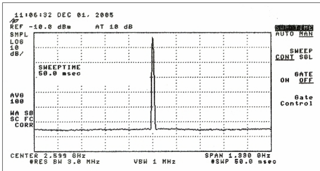
Figure 4-7. Products Above the -62 dB Noise Floor of the Spectrum Analyzer (1.330 GHz Span)
