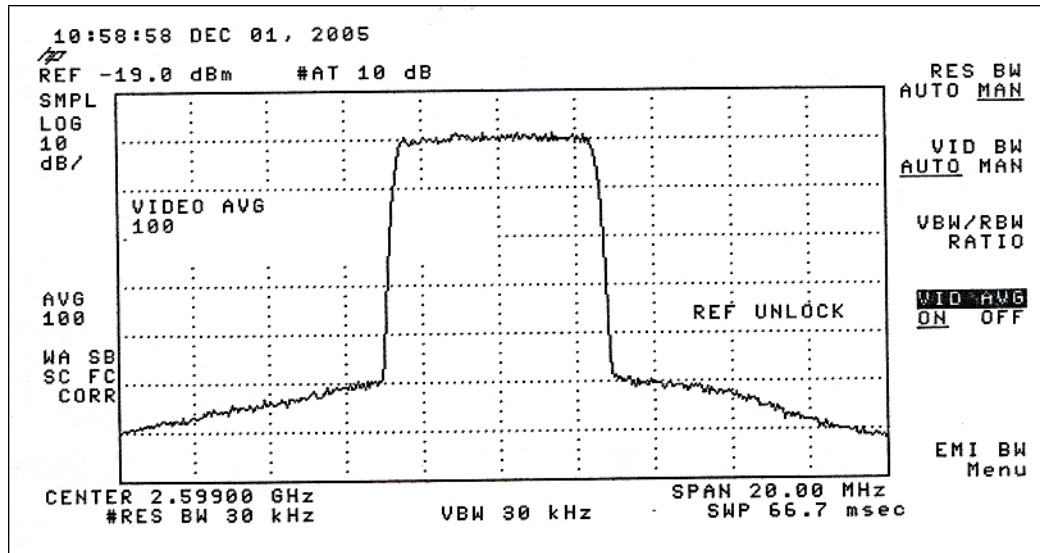
Figure 4-8. Conducted Spurious Emissions (before channel filter)
