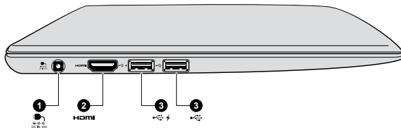
Figure 3-2 The left side of the computer
