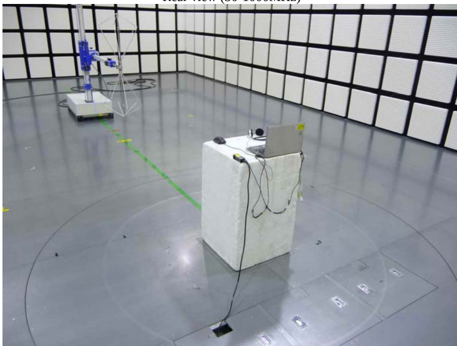
Rear view (30-1000MHz)
