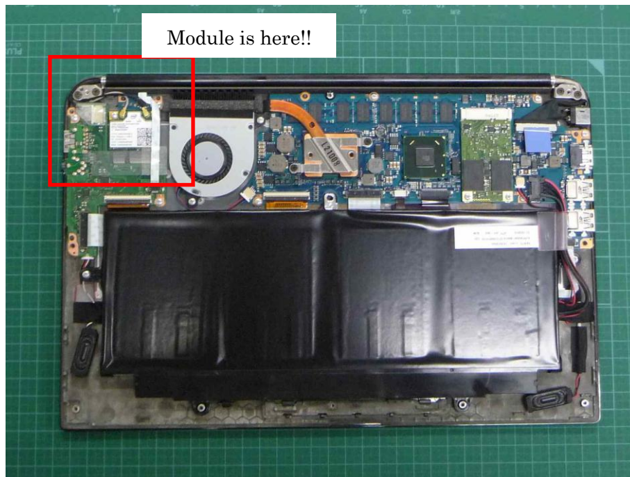
Bottom cover removed
