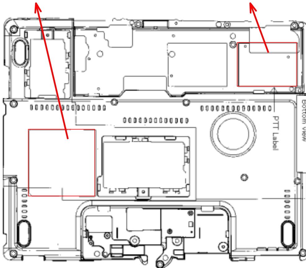
[Bottom view]
