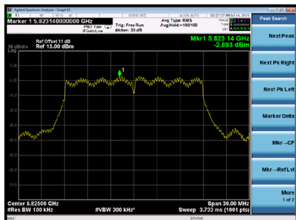
Channel 165 (5825MHz)
