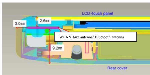
Top side view(WLAN Aux antenna/ Bluetooth antenna)
