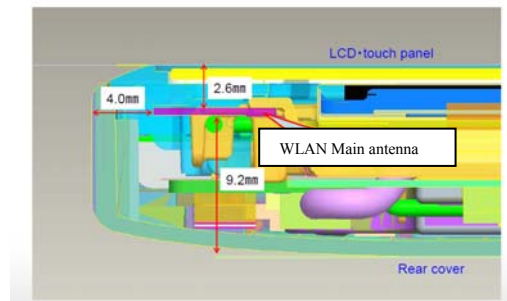
Top side view(WLAN Main antenna)
