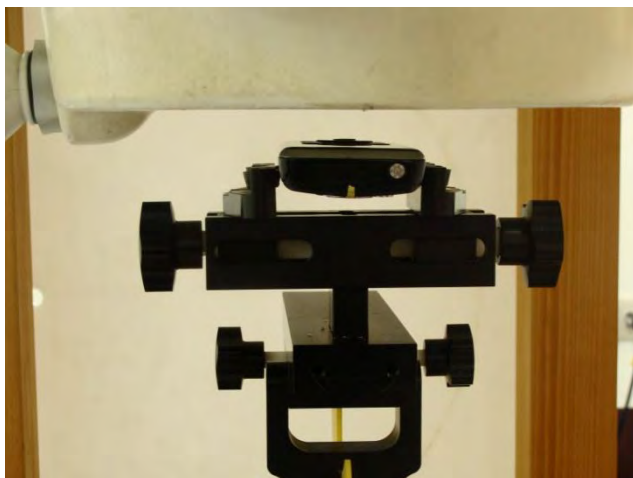
Front Face of the DUT with Phantom 1.5 cm Gap
