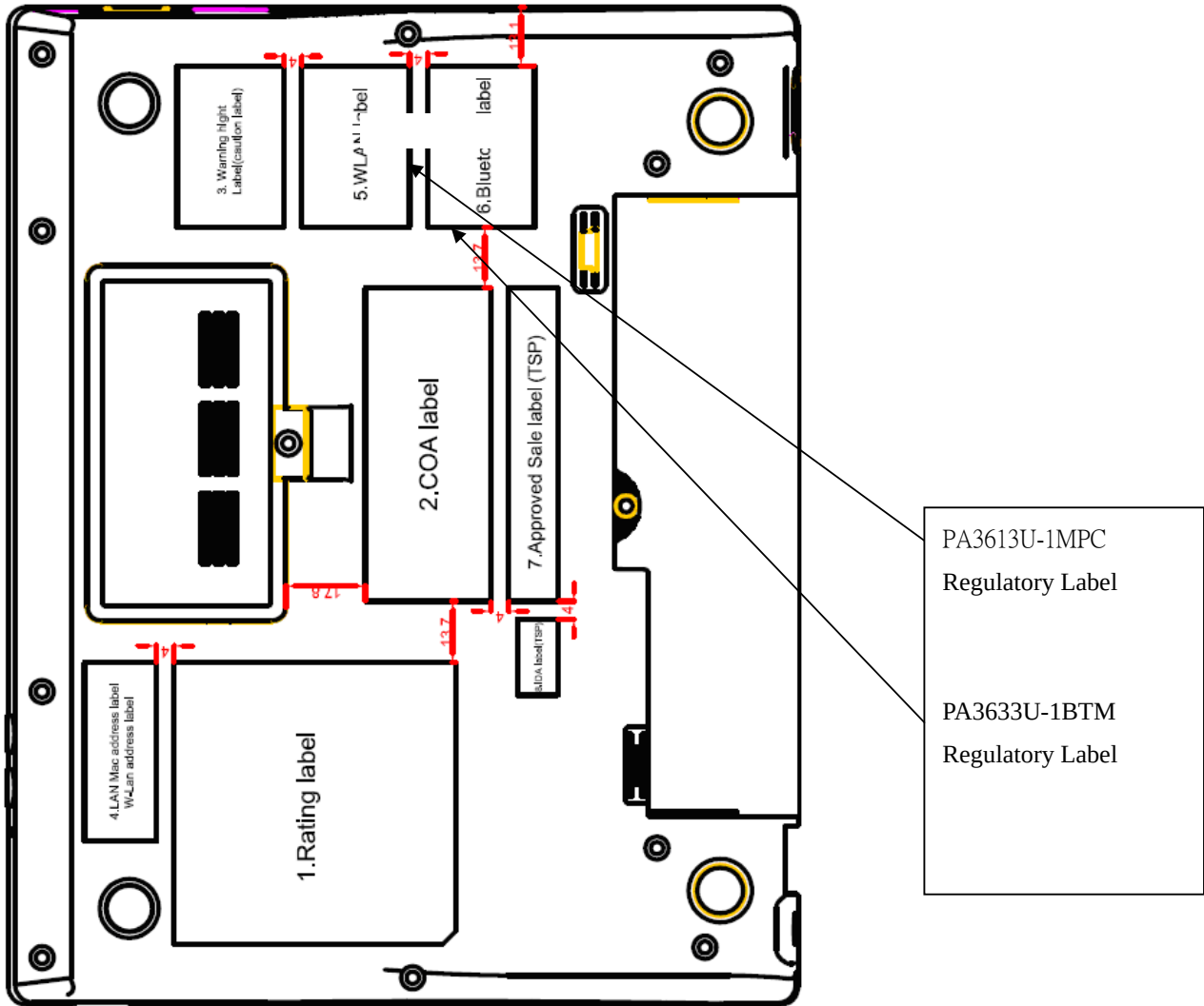
Regulatory Label of PA3613U-1MPC on bottom of PC
