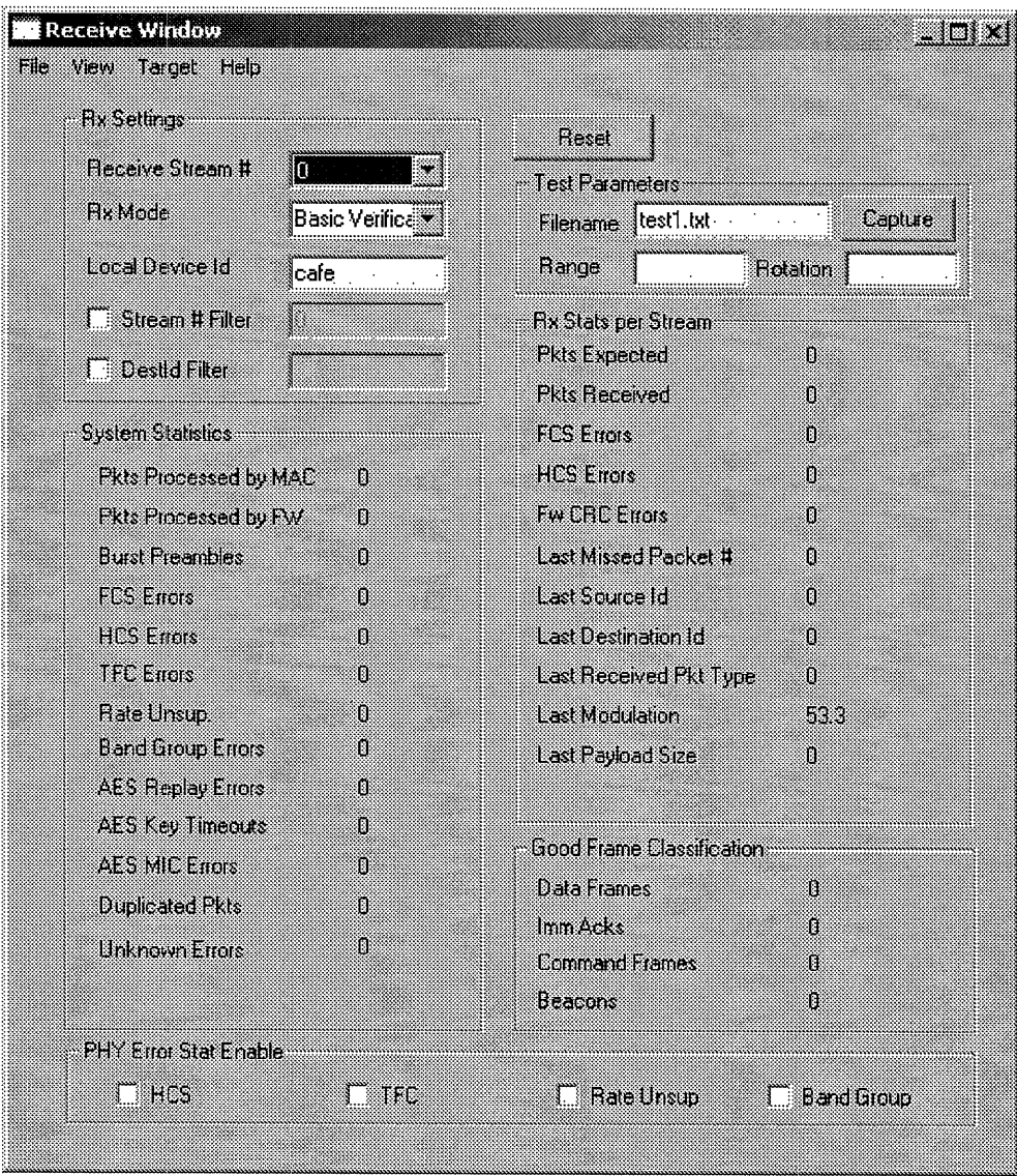
Figure 23 - Receive Window
