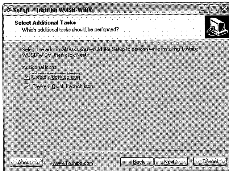
Figure 8 - Select Components
