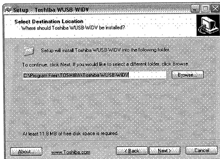
Figure 6 - Information Window
