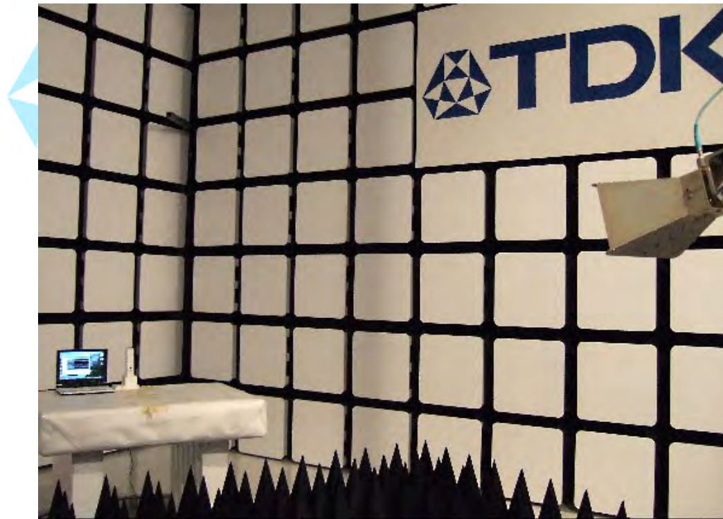
Test Configuration 2: 3 GHz to 5 GHz
