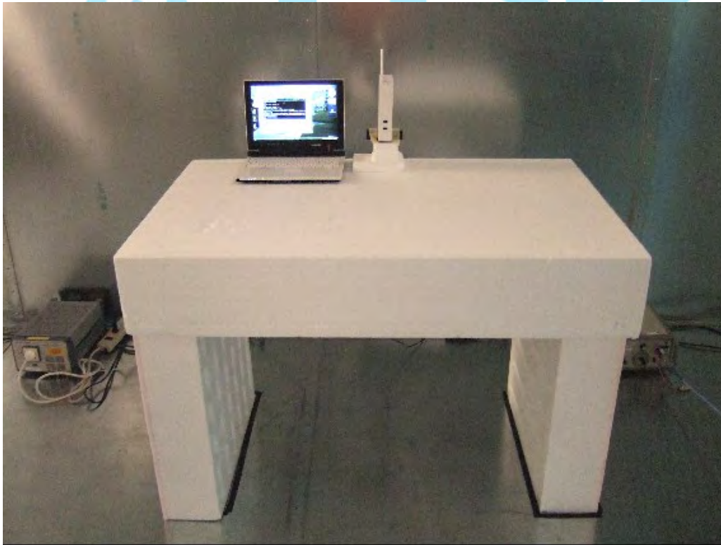
Test Configuration 4: AC conducted
