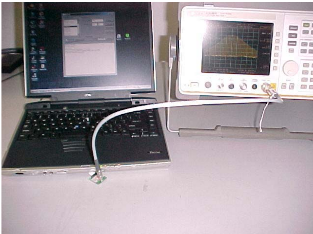
Conducted Emissions at Antenna Terminal Setup
