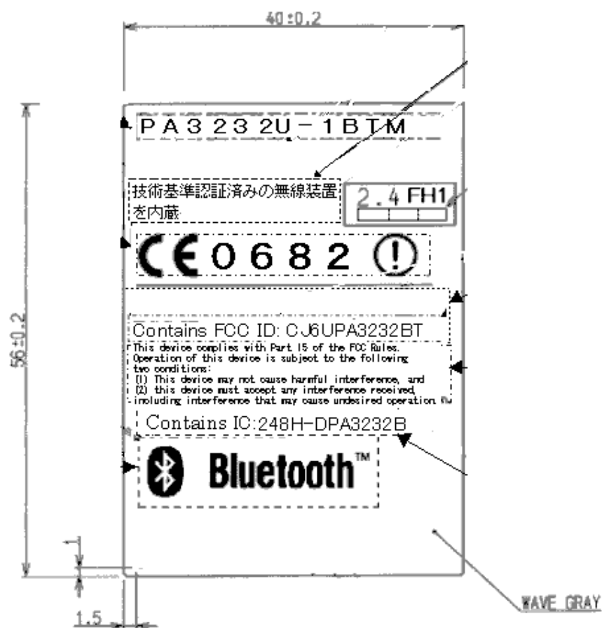
Bluetooth label
