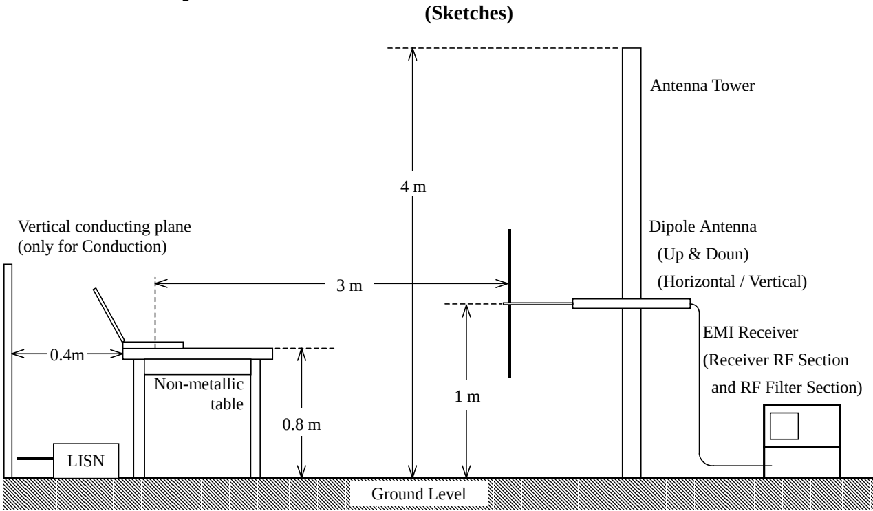
Figure 1, Side View
