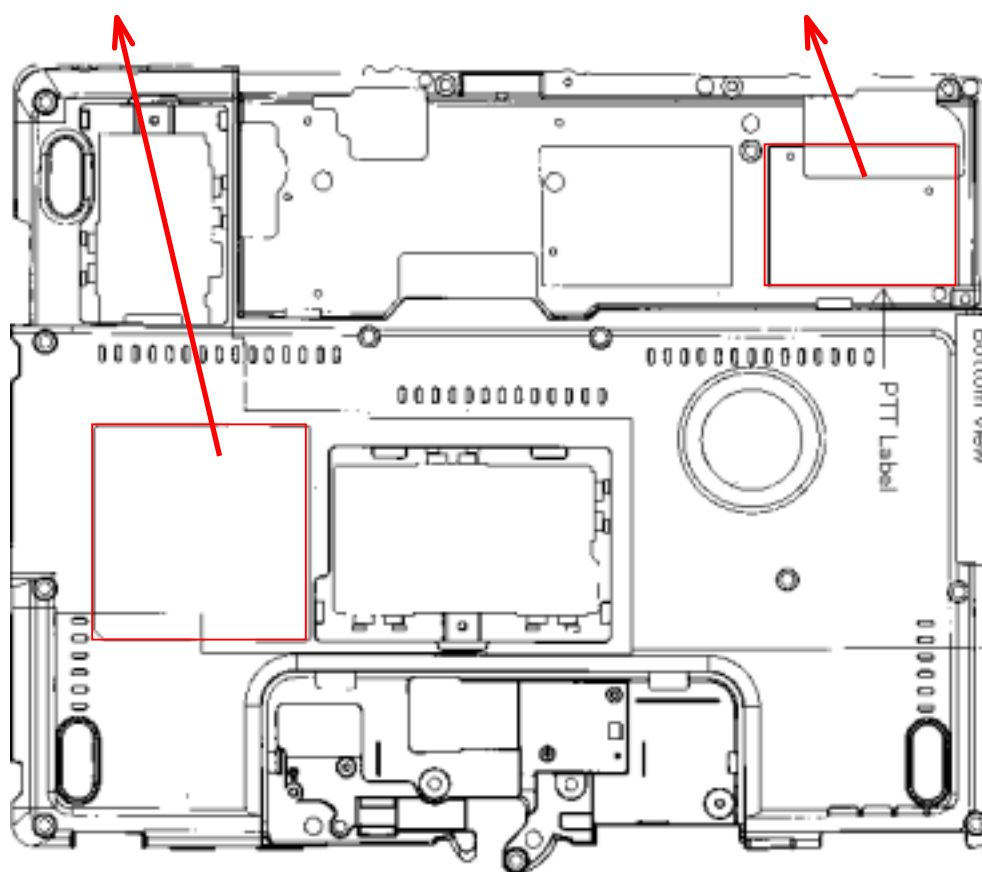
[Bottom view]
