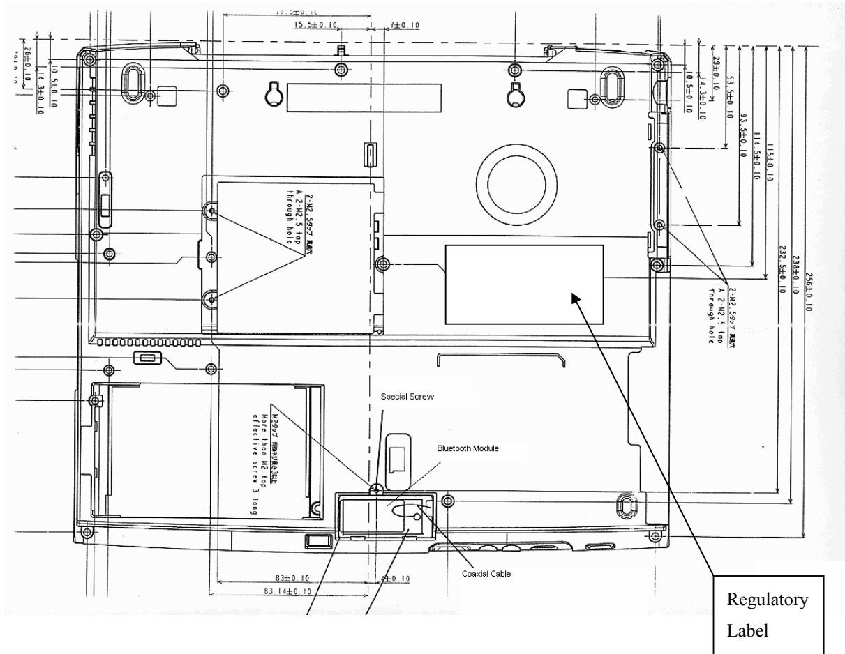
Bottom side view
