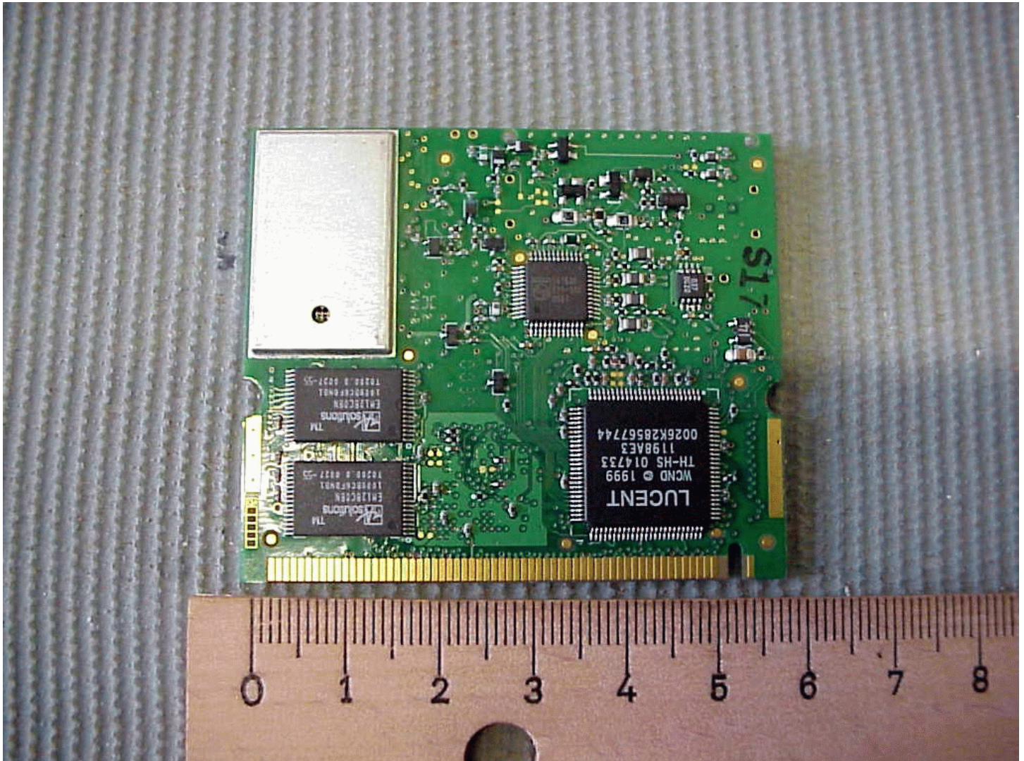
Mini PCI Wireless LAN board - lower side with shield
