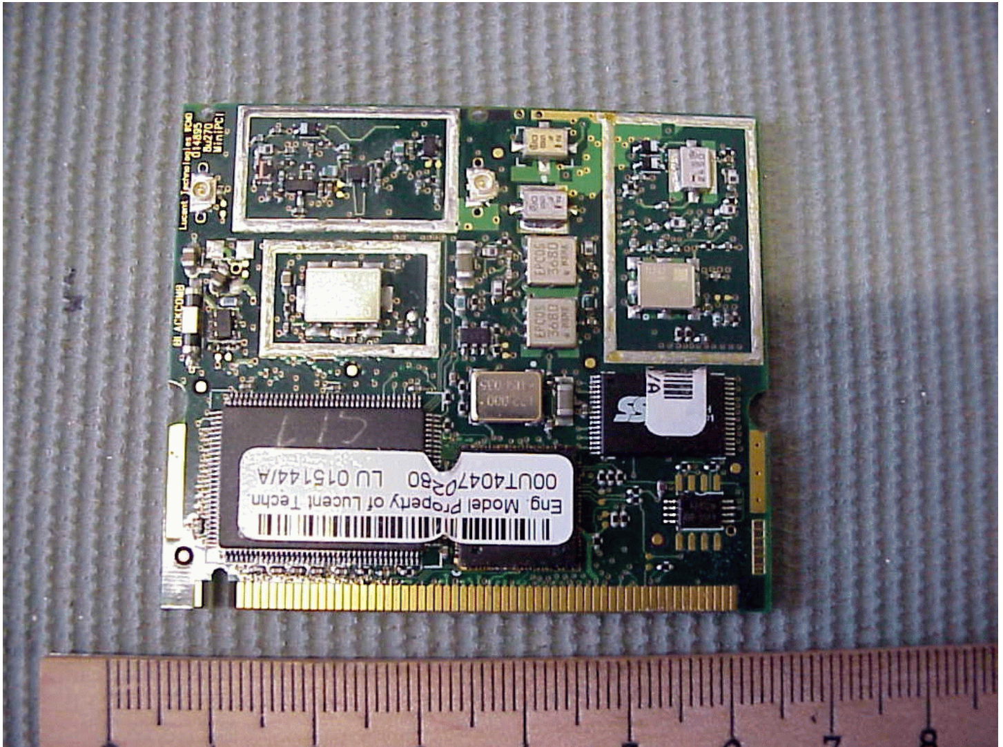
Mini PCI Wireless LAN board - upper side without shield
