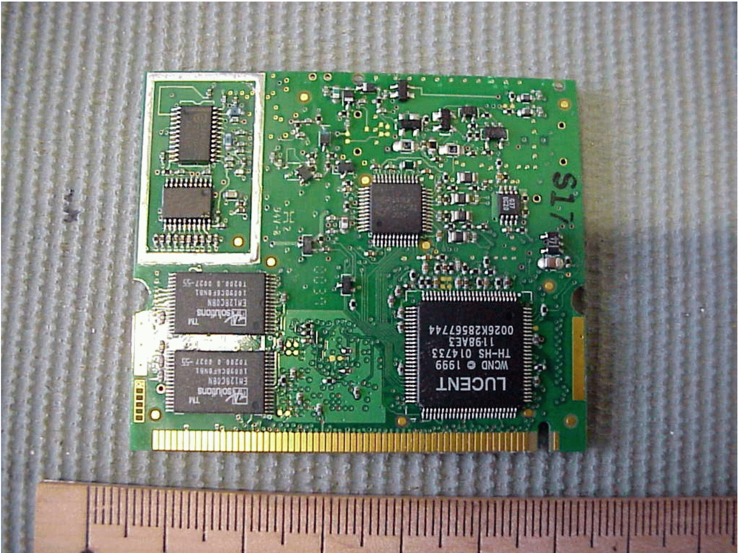
Mini PCI Wireless LAN board - lower side without shield
