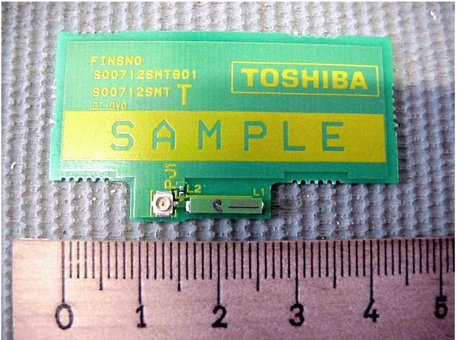
Antenna board, top side
