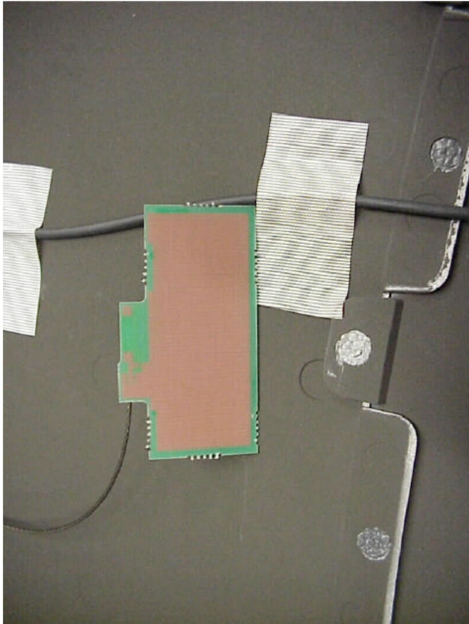
Antenna view backside (Antenna is the same as used in Satellite Pro 4600)
