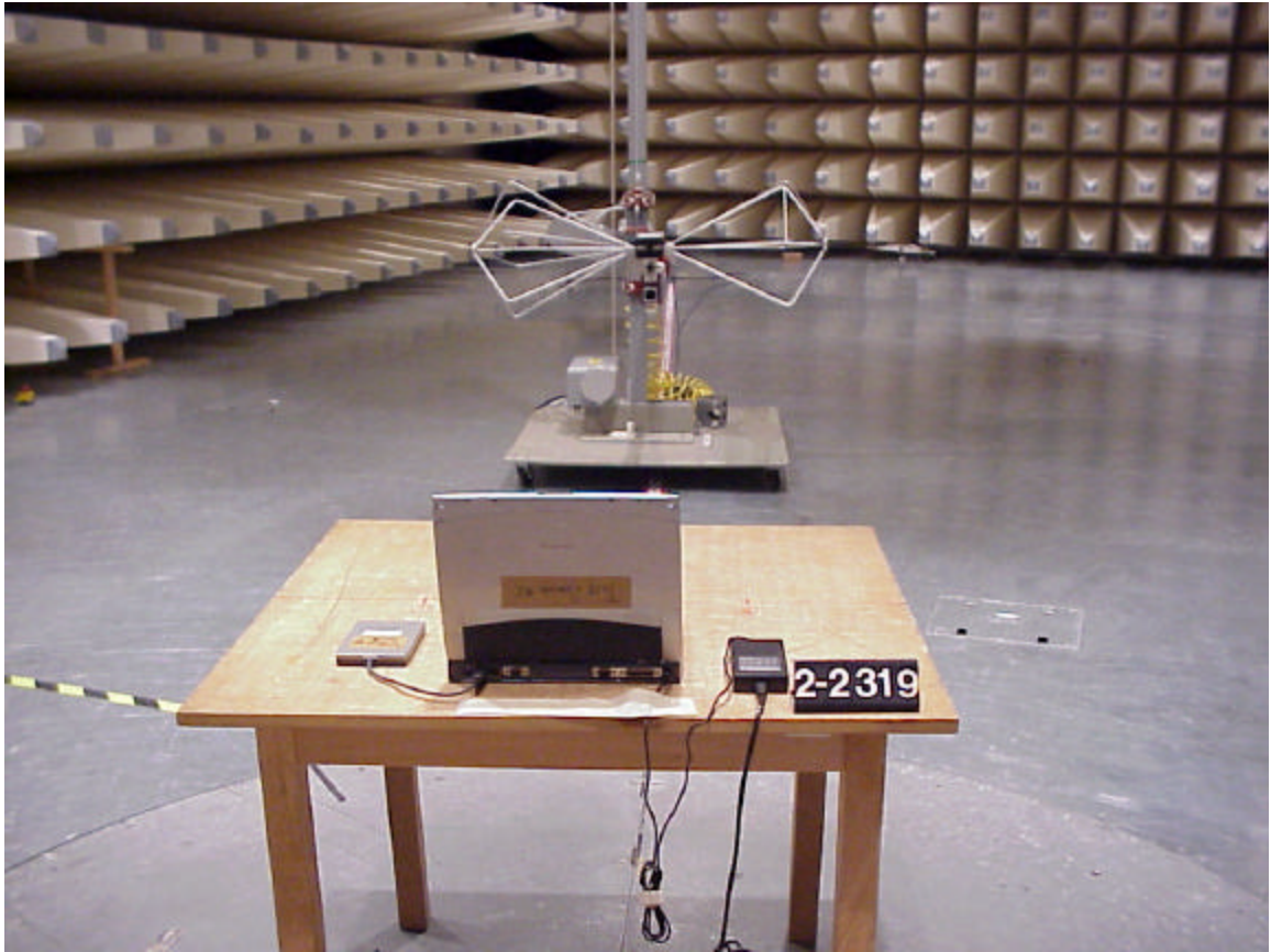
Back close-up view of test setup
