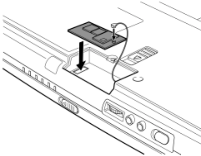
Figure 2 Installing the Bluetooth board
